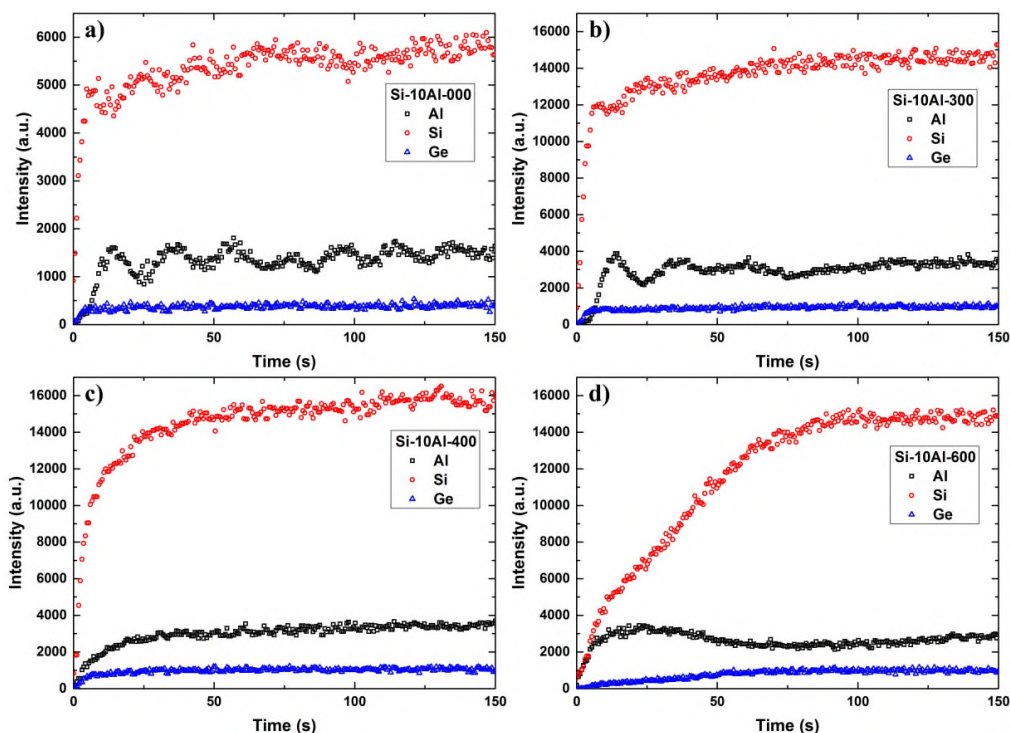
Fig. 2: SNMS depth profiles of sample Si-10Al a) in the as-deposited state and after annealing at different temperatures of b) 300 °C, c) 400 °C, and d) 600 °C.
