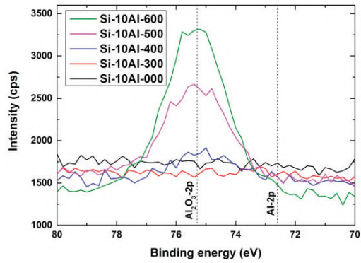
Fig. 3: XPS measurements of the Al-2p peak of sample Si-10Al obtained after different annealing conditions.
