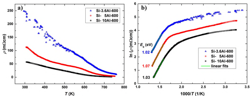
Fig. 5: a) Comparison of the resistance for samples crystallized at an annealing temperature of 600 °C. b) Arrhenius plot of the resistance with linear fits in the high temperature range representing the intrinsic excitation energy of the Si substrate.
