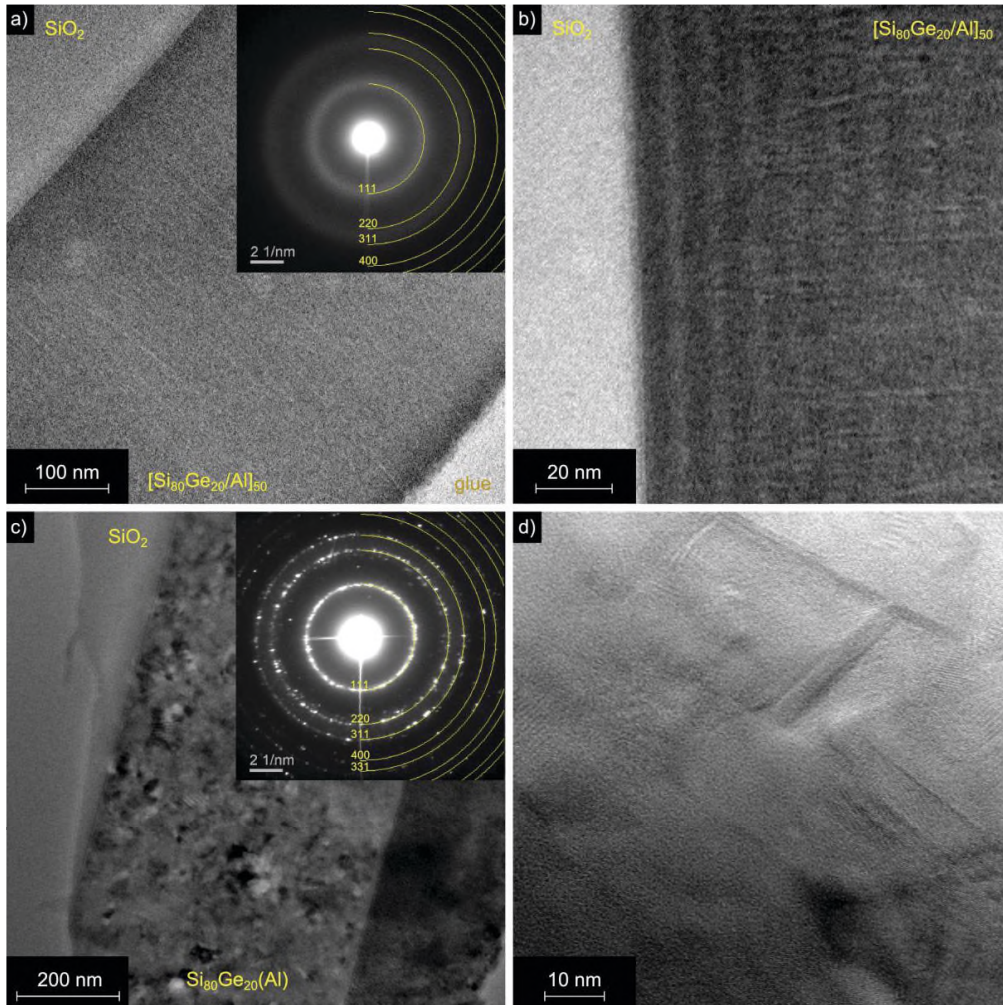
Fig. 1: a), b) TEM bright field images of sample Si-10Al in the as-deposited state and c), d) after annealing at 600 °C at low and high magnifications, respectively. The insets in a) and c) show SADPs taken at the area of the Si 80 Ge 20 with yellow lines representing the theoretical diffraction rings of Si 80 Ge 20 .
