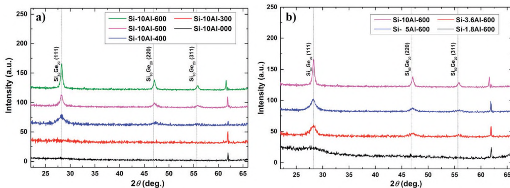
Fig. 4: X-ray ( \theta - 2\theta ) diffractograms of samples annealed a) at different annealing temperatures and b) with varied Al interlayer thickness d_{Al} .
