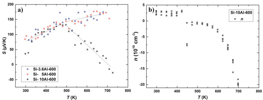
Fig. 6: a) Seebeck coefficient for samples crystallized at 600 °C with guides to the eye added for respective temperature regions. b) Hall effect measurement conducted on sample Si-10Al-600.
