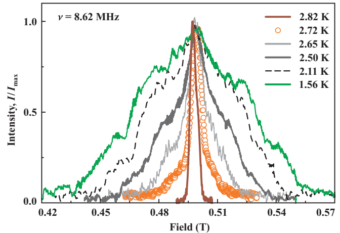
FIG. 17. (Color online) Temperature-dependent ^{31}\text{P} NMR spectra measured at \nu = 8.62 MHz.
