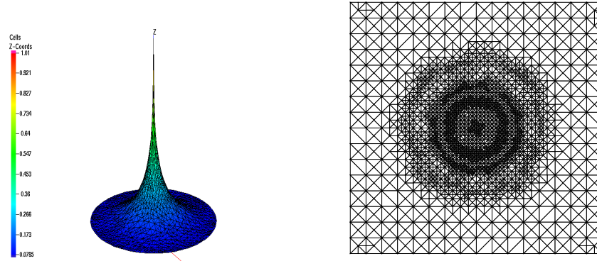
Fig. 2. Optimal adjoint state (left) and adaptively refined triangulation after 14 refinement steps of the adaptive loop (right)
