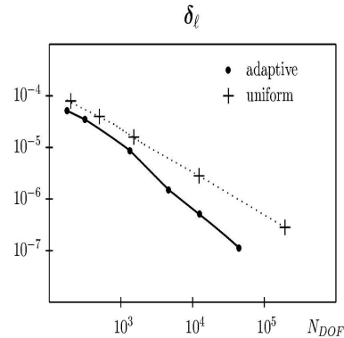
Fig. 3. Decrease of the quantity of interest \delta_\ell := |J(y, u) - J_\ell(y_\ell, u_\ell)| as a function of the total number of degrees of freedom for adaptive and uniform refinement
