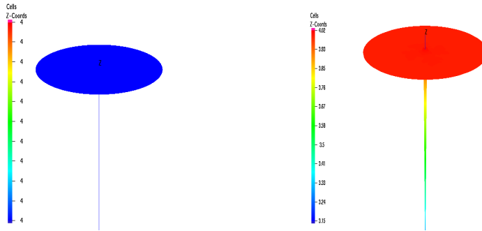
Fig. 1. Optimal state (left) and optimal control (right)
