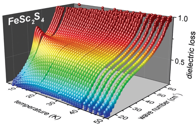
FIG. 2. (Color) Three-dimensional plot of the dielectric loss of FeSc 2 S 4 vs wave number and temperature. The loss is color coded to indicate equal-loss contours above the temperature wave-number plane.
