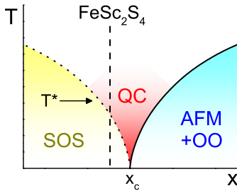
FIG. 1. (Color online) Schematic x, T phase diagram based on theoretical considerations [1,11] (see text for details). The control parameter x measures the ratio of the magnetic exchange to the effective spin-orbit coupling. SOS, QC, AFM, and OO denote spin-orbital singlet, quantum-critical, antiferromagnetic, and orbitally ordered states, respectively. The vertical dashed line indicates the position of \text{FeSc}_2\text{S}_4 .
