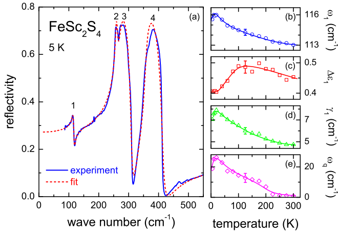
FIG. 4. (Color online) (a) FIR measurements between 80 and 600\text{ cm}^{-1} are compared with a fit utilizing four Lorentz oscillators. The four phonon modes are indexed from 1 to 4. The right frames show the temperature dependence of eigenfrequency \omega_0 (b), dielectric strength \Delta\epsilon (c), damping \gamma (d), and the Fano factor \omega_q (e) of phonon 1 close to 115\text{ cm}^{-1} . In (b)–(e), typical error bars are indicated. The solid lines are drawn to guide the eyes.
