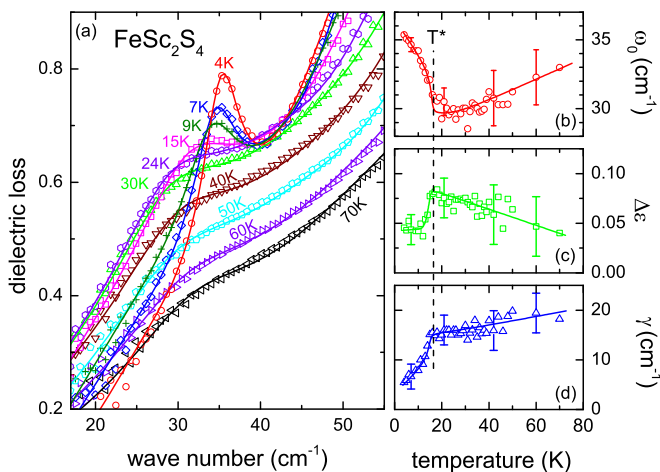
FIG. 3. (Color online) (a) Dielectric loss of FeSc 2 S 4 at low wave numbers for selected temperatures between 4 and 70 K. The solid lines represent fits using Lorentzian line shapes including a temperature-dependent background (see text). Right column: Temperature dependence of eigenfrequency (b), of the dielectric strength (c), and of the damping constant (d) of the spin-orbiton. The solid lines in (b)–(d) serve as guides to the eye. The dashed vertical line indicates a temperature T^* \approx 17 K, below which a change of the characteristics of the excitation is observed.
