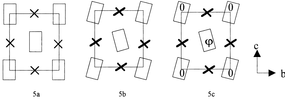
Fig. 5. Schematic representation of the projection along a direction of the structure of the (FA)_2PF_6 at RT (a), between T_c and T_p (b) and below T_p (c). \phi is the phase shift between 1 st neighbouring CDWs. The FA stacks are represented by open rectangles and the PF_6^- anions by crosses.
