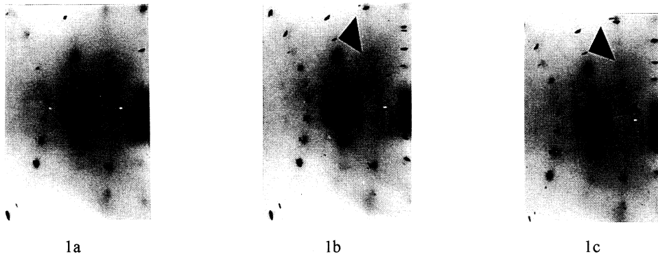
Fig. 1. X-ray patterns of (FA)_2PF_6 at 300K (a), 190K (b) and 175K (c). The chain axis a is horizontal.
