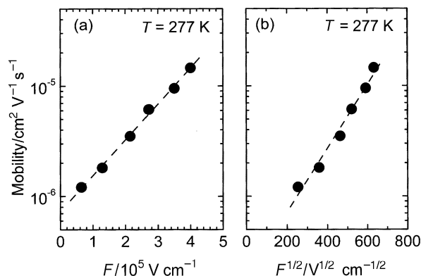
Fig. 10 Dependence of the drift mobility in PPV at T = 277 \text{ K} on (a) the electric field (polaron hopping model) and (b) the square root of the electric field (Poole–Frenkel model). Reprinted with kind permission from ref. 24.
