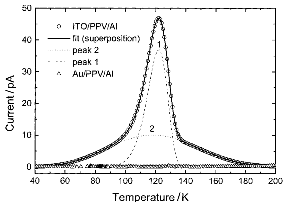
Fig. 6 Comparison of TSC spectra of an ITO/PPV/Al and a Au/PPV/Al device. Both samples were measured simultaneously after identical trap filling. The spectrum of the ITO device can be fitted by a superposition of two peaks. Reprinted with kind permission from ref. 23.
