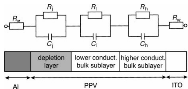
Fig. 2 Equivalent circuit used to model the behaviour of the dielectric function shown in Fig. 1.
