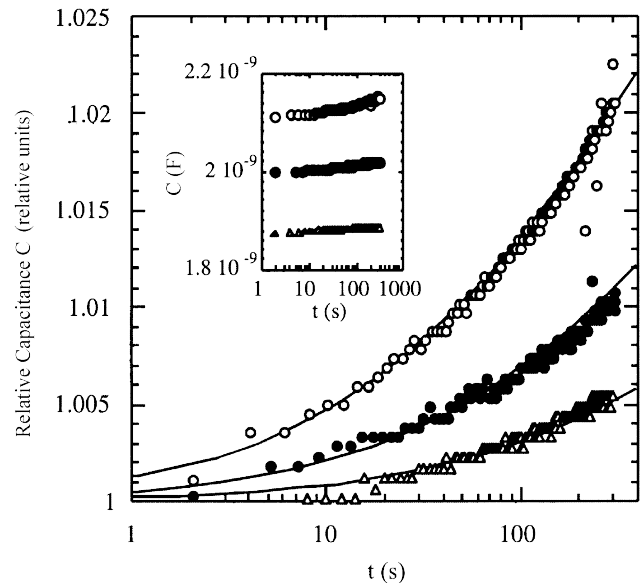
Fig. 4. Variation of relative capacitance, C_{\text{rel}} , against time, t , at 300 K (open circles), 280 K (filled circles) and 260 K (open triangles). Solid lines are fits to model at these temperatures for \sigma = 0.10 eV, E_t = 0.75 eV, \nu = 10^8 \text{ s}^{-1} and N_t = 6.0 \times 10^{17} \text{ cm}^{-3} . Data and fits have been normalised to C of fits at t = 10^{-5} s for illustration purposes. Insert shows unnormalised original data.
