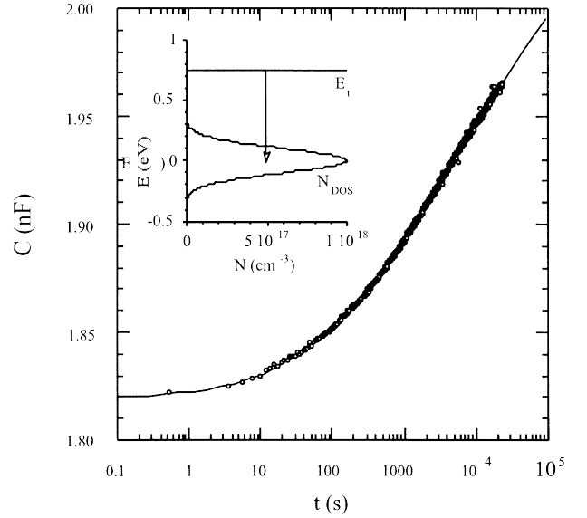
Fig. 3. Fit of model to results in Fig. 2 on a lin-log plot. Parameters used in fit are \sigma = 0.10 eV, E_t = 0.75 eV, \nu = 10^8 s ^{-1} and N_t = 5.1 \times 10^{17} cm ^{-3} . Inset shows physical picture of decay model.
