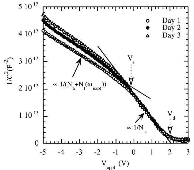
Fig. 1. Inverse capacitance squared, 1/C^2 , against applied bias, V_{\text{appl}} , of a 200 nm thick ITO/PPV/Al device. Recorded at 1 day intervals in He atmosphere after exposure to air.
