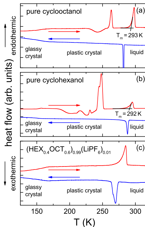
FIG. 1. DSC measurements on cooling (lower lines) and heating (upper lines) with rates of 10 K/min for pure cyclooctanol (a) and pure cyclohexanol (b), compared with the mixture (HEX 0.4 OCT 0.6 ) 0.99 (LiPF 6 ) 0.01 (c). Endothermic processes are plotted in the positive y-direction. Three different phases are assigned to the cooling measurements as they sequentially occur on cooling: liquid, plastic crystal, and glassy crystal.
