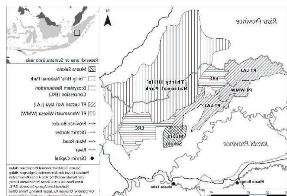
Figure 4: Research Area – Bukit Tigapuluh/30 Hills Landscape
