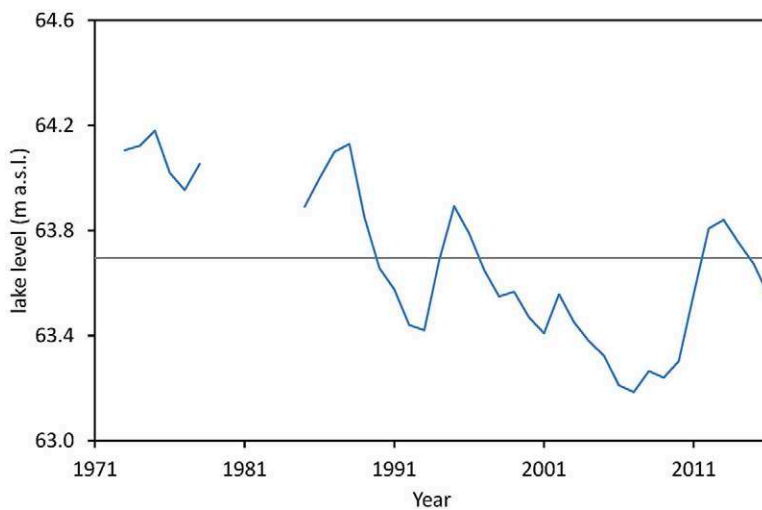
Fig. 2. Lake level of Lake Füstenseer See, 1972 to 2016 (source: State Agency for Agriculture and Environment, Mecklenburg Lake District).
