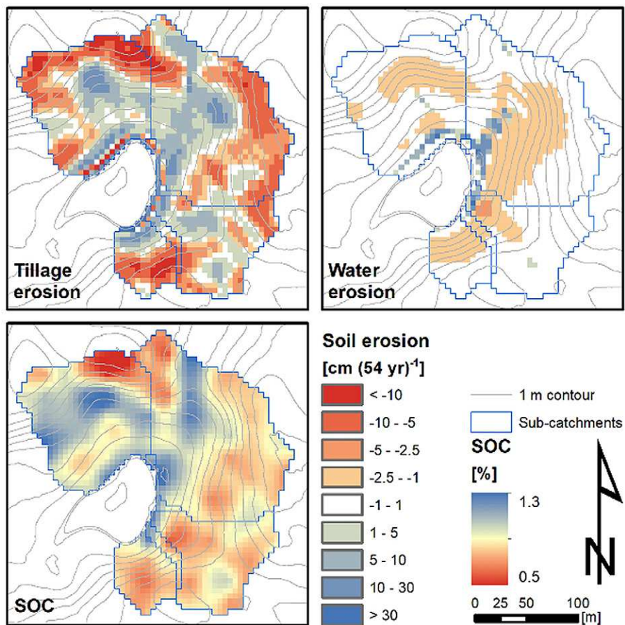
Fig. 16. Spatial distribution of topsoil soil organic C (SOC) and modeled tillage and water erosion in the monitored kettle hole at Christianienhof over 54 yr; negative and positive values of erosion indicate soil loss and gain, respectively.
