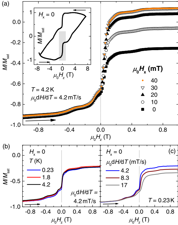
FIG. 1. Spin reversal in transverse fields for \text{Li}_2(\text{Li}_{0.994}\text{Fe}_{0.006})\text{N} ( M \parallel H_z \parallel c ). Shown are sections of isothermal M-H half loops. (a) The step in M at H_z \approx 0 roughly doubles its size in a transverse field of \mu_0 H_x = 30 mT. A full M-H loop is given as inset. Compared to an applied transverse field, the effects of temperature and sweep rate on the step-size are small as shown in (b) and (c), respectively.
