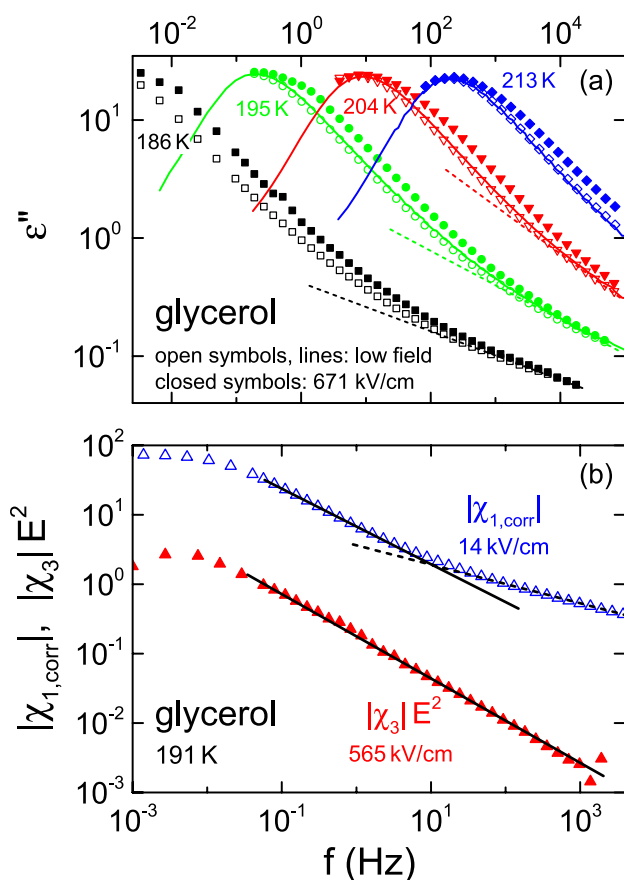
Figure 5. (a) Dielectric loss of glycerol measured at fields of 14\text{ kV cm}^{-1} (open symbols) and 671\text{ kV cm}^{-1} (closed symbols) shown for four temperatures [31]. The solid lines were measured with 0.2\text{ kV cm}^{-1} [30]. The dashed lines indicate the excess wing. (b) Open triangles: absolute values of \chi_1 (corrected for \chi_{1,\infty} = \epsilon_\infty - 1 ) at 14\text{ kV cm}^{-1} for glycerol at 191 K. Closed triangles: \chi_3^{(3)}E^2 at 565\text{ kV cm}^{-1} [34]. The solid lines indicate similar power laws above the peak frequency for both quantities. The dashed line indicates the excess wing in the linear susceptibility at high frequencies, which has no corresponding feature in \chi_3^{(3)}(\nu) .
