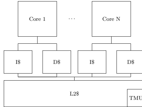
Fig. 1. The multicore system we consider consists of up to 16 cores. Each core has a private L1 instruction cache as well as a private L1 data cache. The TMU is integrated into the L2 cache and is able to monitor the messages relevant for the transactional execution.
