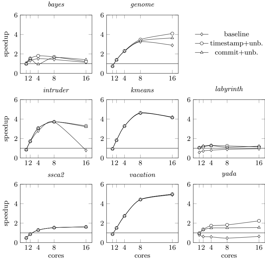
Fig. 2. Results of the execution of the STAMP benchmark suite [6]. For five of the benchmarks we were able to achieve speedups. For the benchmarks genome, intruder and yada we improved performance compared to the baseline implementation.
