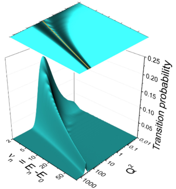
FIG. 3. Transition probability T(\nu_n, Q^2) computed for the confining potential with \eta = 2 in the presence of the Coulomb interaction. The scaling direction is seen by projection into the (\nu_n, Q^2) plane.
