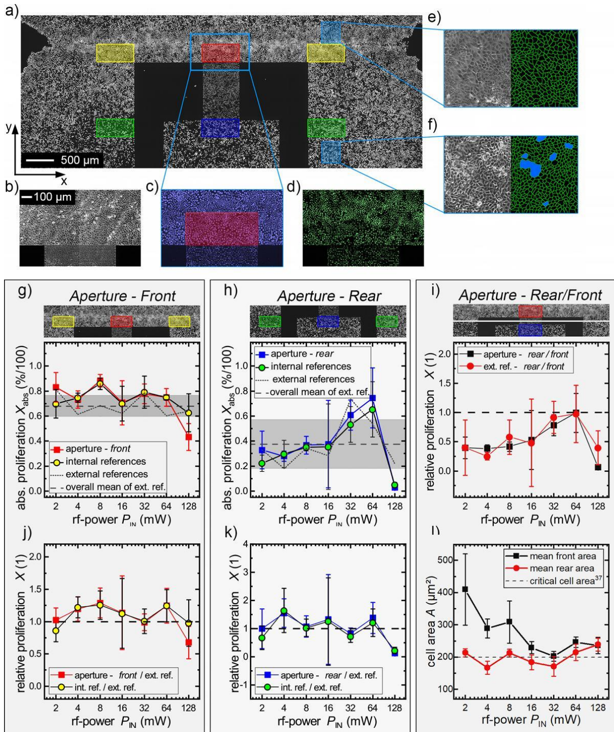
Figure 5: Determination of the SAW-induced influence on cell proliferation. a) Fluorescence image of nuclei with newly synthesized DNA with evaluated regions marked in different colors (red: front aperture, yellow: internal reference front, blue: rear aperture, green: internal reference back). b) – d): Images of the artificial wound in phase contrast (b)), all cellular nuclei (c)) and newly synthesized (d)). e)/f) Phase contrast images and cell border of the cell layer. e) MDCK-II at low density (wound) f) MDCK-II at high density with emerging cell domes (blue spots). g)/h) Absolute proliferation X_{\text{abs}}(P_{\text{IN}}) of the front and rear area. i) Relative proliferation inside the cell layer and at the edge. j)/k) SAW-stimulated samples compared to external references. l) Average area per cell in the corresponding external reference in the front and rear section of the aperture. Cultivation time for measurement point at P_{\text{IN}} = 16 mW t = 22 h, else t = 27 h.
