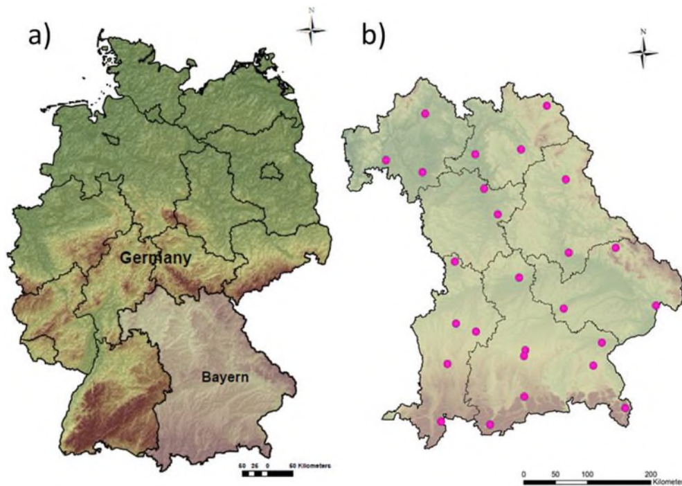
Fig. 1. Bavaria (Germany). Pollen monitoring locations in Bavaria only.
