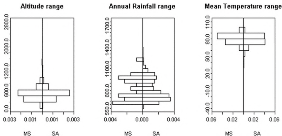
Fig. 2. Studied range of environmental conditions over the 26 monitoring stations (MS) and over the study area (SA), Bavaria (Germany). Variables: Altitude (m.a.s.l.), Annual rainfall (mm) and Annual Mean Temperature ( ^{\circ}\text{C}\cdot 10 ).
