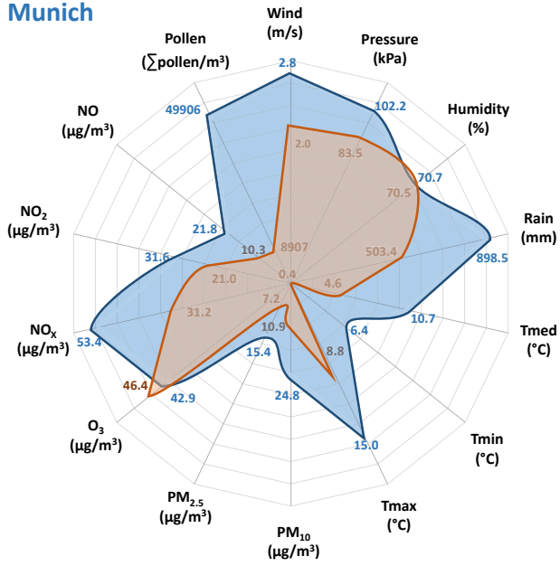
FIG E1. Kiviatic diagram of the average of yearly averages of weather/aerosol daily values during the study period (2012-2015) in the atmosphere of Munich (Germany) and Davos (Switzerland).
