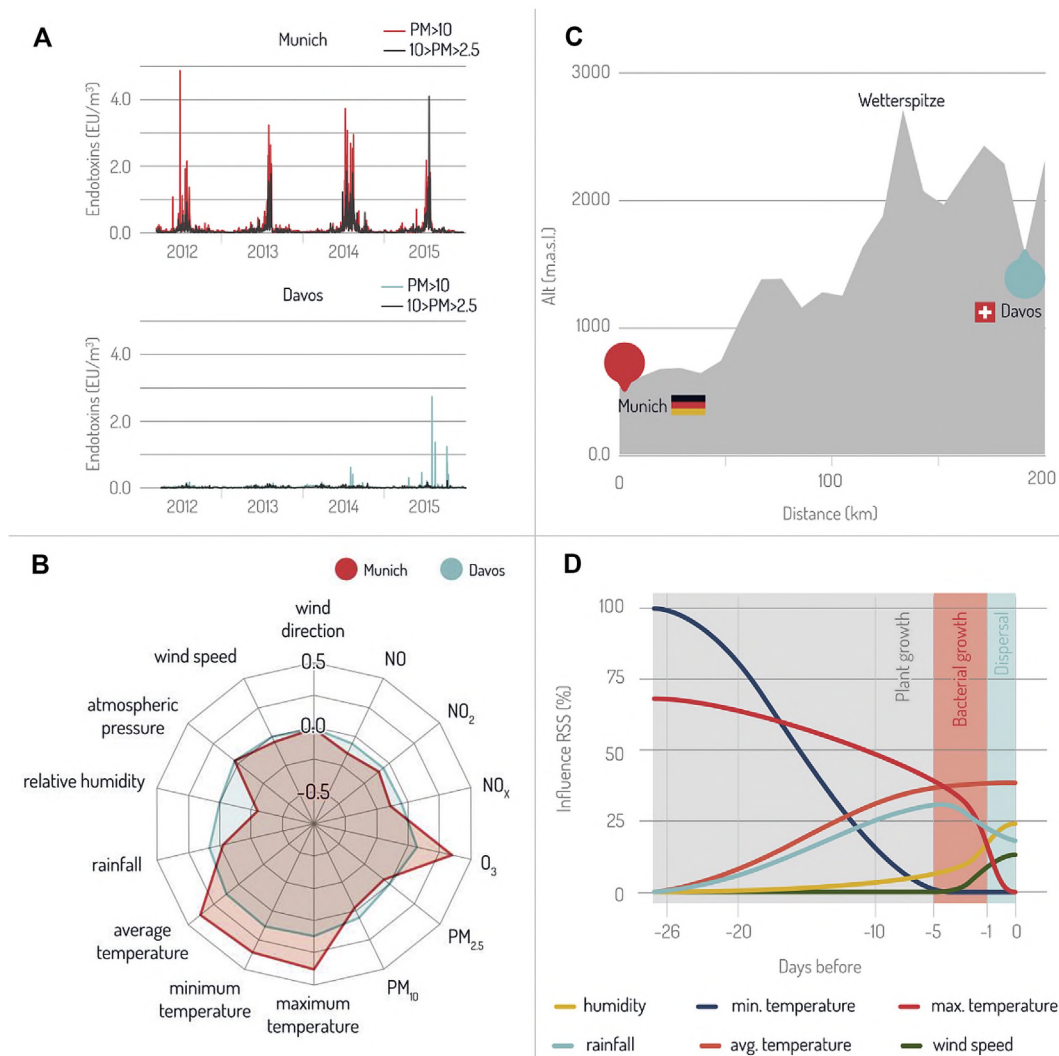
FIG 1. A , Daily endotoxin concentrations determined with the rFC method in Munich and Davos (2012-2015). Endotoxin concentrations were measured in 2 fractions of ambient air: PM >10 and 10>PM >2.5 . B , Kiviat diagram with Pearson correlations between daily endotoxin concentrations and weather variables/aerosols in the atmosphere in Munich (Germany) and Davos (Switzerland). No correlation was at an r value of greater than 0.5, and the represented correlation range is between -0.5 and 0.5 (all P > .05 ). No correlation of greater than 0.5 existed with 30 different types of airborne pollen (data not shown). C , Altitude gradient between monitoring locations in central Europe: Davos (Switzerland) and Munich (Germany). D , Variables for forecasting daily endotoxin concentrations by using residual sum-of-square values at each of the 3 MARS models: model A (plant growth), model B (bacterial growth), and model C (pollen dispersal). Model A (explained 50% of variance) is based on weather conditions during day -26 to day -5 before the forecasted day. Model B (explained 59%) is based on model A plus weather conditions during the period from day -4 to day -1. Model C (explained 71%) is based on model B plus weather conditions on the forecasting day.
