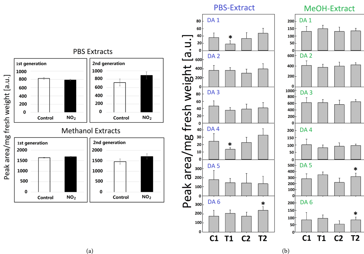
Figure 2. (a) Total amount of water-soluble and methanol-extractable phenolic metabolites in ragweed pollen. The separation was performed by RP-HPLC. Plants were fumigated with 40 ppb NO 2 (1 st control) or clean air (2 nd control) or with 80 ppb NO 2 (1 st and 2 nd treatment); bars indicate \pm SD; N = 8 plants, 5 inflorescences per plant). (b) Amount of individual PBS-soluble and methanol-extractable phenolic metabolites in pollen of A. artemisiifolia . C1 = 1 st population of control; T1 = 1 st population of treatment; C2 = 2 nd population of control; T2 = 2 nd population of treatment. The bars indicate \pm SD and significant differences are indicated by asterisks (N = 8 plants, 5 inflorescences per plant; t-test, *p-value < 0.05).
