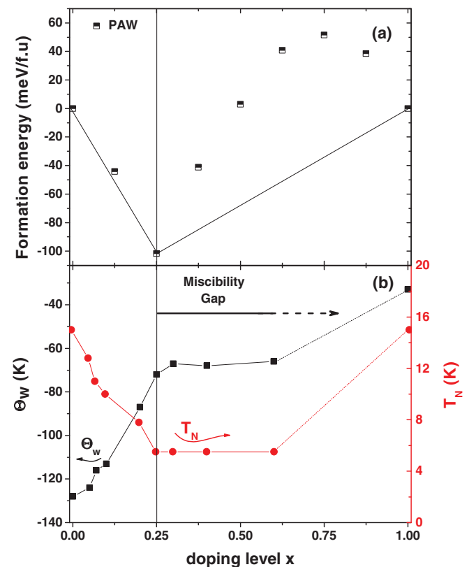
FIG. 8. (Color online) (a) Phase diagram of (\text{Na}_{1-x}\text{Li}_x)_2\text{IrO}_3 obtained from spin-polarized GGA + SOC + U total energy calculations. Shown are the formation energies obtained with the PAW basis. The vertical line indicates the composition at x = 0.25 , which is a very stable \text{Na}_3\text{LiIr}_2\text{O}_6 structure with alternating \text{LiIr}_2\text{O}_6 and \text{Na}_3 layers. (b) Phase diagram with T_N and CW temperature \theta_w of (\text{Na}_{1-x}\text{Li}_x)_2\text{IrO}_3 , data at x = 1 are from Ref. [10]. The miscibility gap region is indicated by the horizontal arrow.
