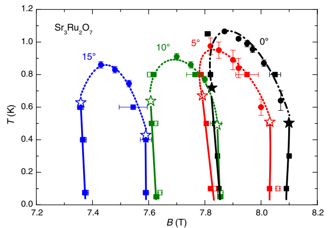
FIG. 4 (color online). Phase diagram of the nematic phase of \text{Sr}_3\text{Ru}_2\text{O}_7 at different tilt angles (cf. different colors). The squares and circles denote transitions in magnetostriction and thermal expansion, respectively (solid symbols: \Delta L \parallel B_{\text{in-plane}} , open symbols: \Delta L \perp B_{\text{in-plane}} ). The black solid lines indicate first-order transitions ending at tricritical points (cf. filled stars) [8], connected by a (dash-dotted) line of second-order transitions. The colored open stars denote the presumed position of critical points, connected by crossover lines (dotted).
