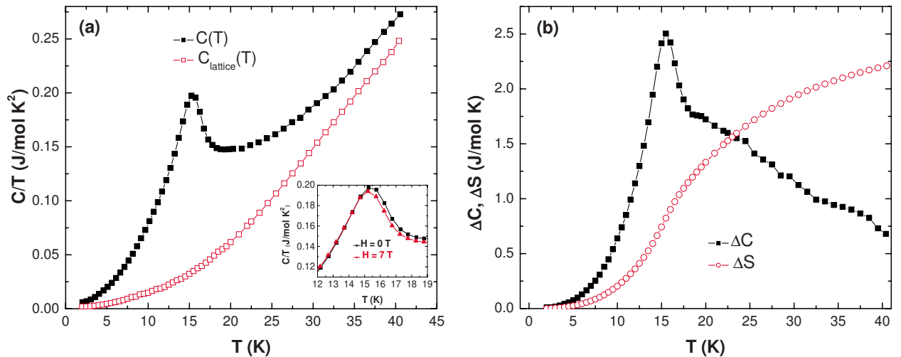
FIG. 6. (Color online) (a) The heat capacity divided by temperature C/T versus T data between T=1.8 K and 40 K for single crystals of \text{Na}_2\text{IrO}_3 and the heat capacity of \text{Na}_2\text{SnO}_3 as the lattice contribution C_{\text{lattice}}/T versus T . The inset shows the C/T versus T data in H=0 and 7 T applied magnetic field. (b) The difference heat capacity \Delta C and difference entropy \Delta S versus T data between T=1.8 and 40 K.
