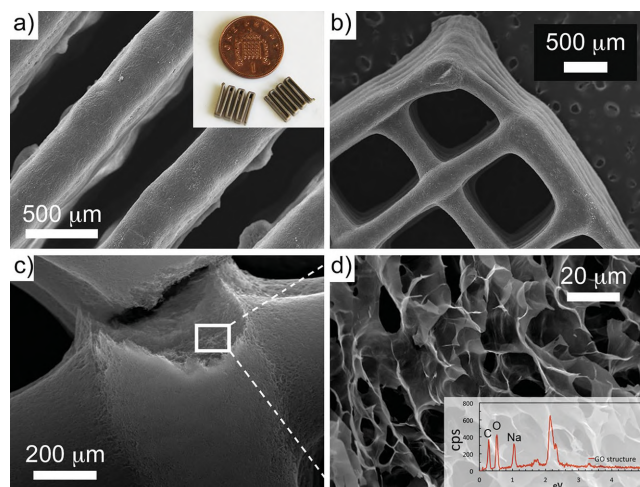
Figure 3. a) Piled up filaments and b) woodpile GO freeze-dried structures (printed through 500 and 150 \mu m nozzles respectively) after drying. The woodpile structure exhibits good bonding between layers and good definition. c,d) Fracture of a junction in a woodpile structure printed through 500 \mu m nozzle showing the inner microstructure of the printed lines. The lines have densities ranging from 25 to 65 mg cm -3 depending on ink formulation (before thermal reduction to rGO). The ice crystals formed during freeze-drying template the formation of a porous architecture inside the printed lines at the microscopic level resulting in highly porous structures with smooth surfaces. The inset in (d) shows an EDS analysis of the freeze-dried structure before reduction. Quantitative EDS analysis before reduction indicate that the dried structures are composed mainly by carbon, oxygen, and small amounts of Na (62% C, 35% O, and 3%Na). Peaks not labeled correspond to the conductive Au coating used for scanning electron microscopy. The sodium impurities come from the NaOH used to regulate the pH during the formulation of the inks.
