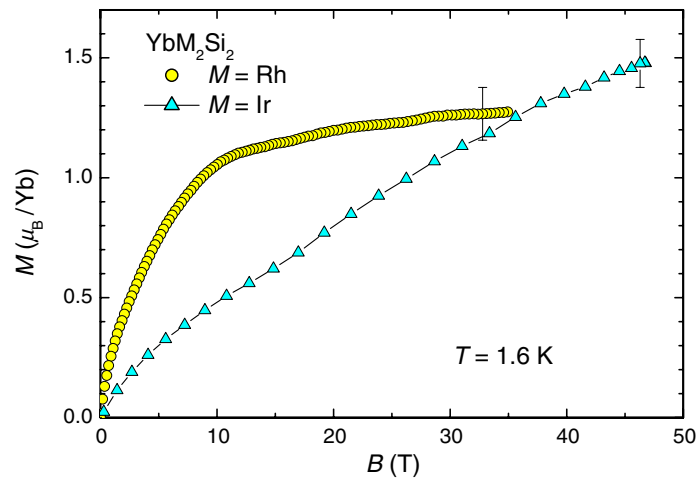
Figure 8. Magnetization M of YbRh 2 Si 2 (yellow circles) and YbIr 2 Si 2 (blue triangles) measured in pulsed fields at 1.6 K on oriented powder samples ( B \perp c ).
