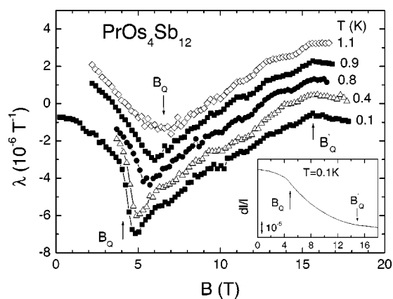
FIG. 3. Linear magnetostriction coefficient \lambda of \text{PrOs}_4\text{Sb}_{12} at various temperatures. For clarity the curves for T>0.1 K were shifted subsequently by 1\times 10^{-6} T -1 . Arrows indicate lower ( B_Q ) and upper ( B'_Q ) boundary of quadrupolar ordered phase. Inset: length change d l/l of \text{PrOs}_4\text{Sb}_{12} vs magnetic field at T=0.1 K.
