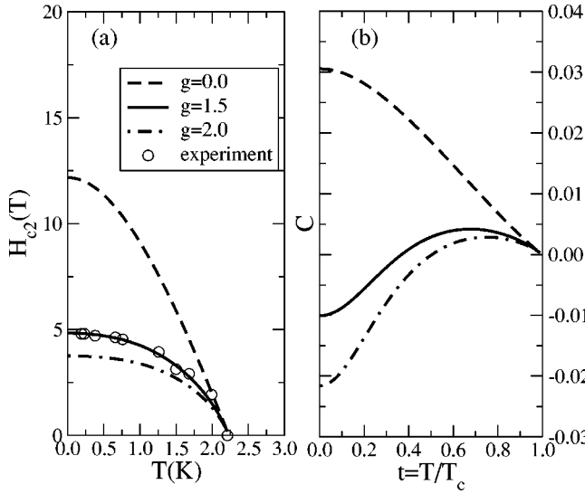
FIG. 1. Temperature dependence of (a) the upper critical field and (b) the admixture parameter C in a d_{x^2-y^2} -wave superconductor with g factors g=0, 1.5, and 2 . The magnetic field is applied along the crystal c direction.
