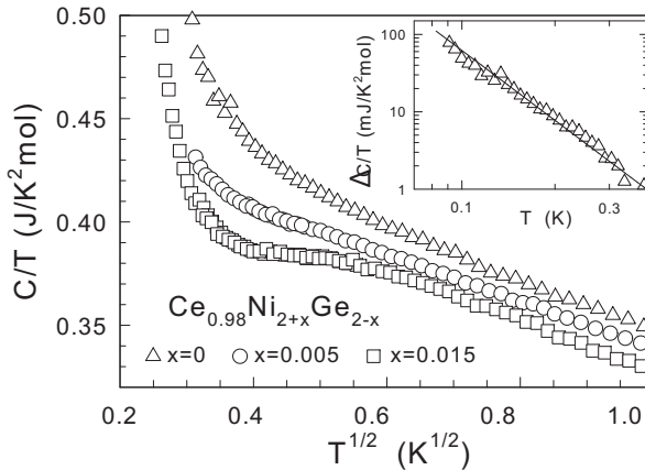
Fig. 1. Low-temperature specific heat of slightly off- stoichiometric \text{CeNi}_2\text{Ge}_2 polycrystals with various starting chemical composition. Inset: \Delta C(T)/T = C(T)/T - (\gamma_0 - \alpha T^{1/2}) for the x = 0 sample on a double-logarithmic scale below 0.4 K. \gamma_0 = 472 mJ/K 2 mol and \alpha = 125 mJ/K 5/2 mol were approximated from the temperature range 0.35 \div 1 K. The solid line displays a \Delta C(T) = AT^{-2} fit with A = 62 \mu\text{JK}/\text{mol} .
