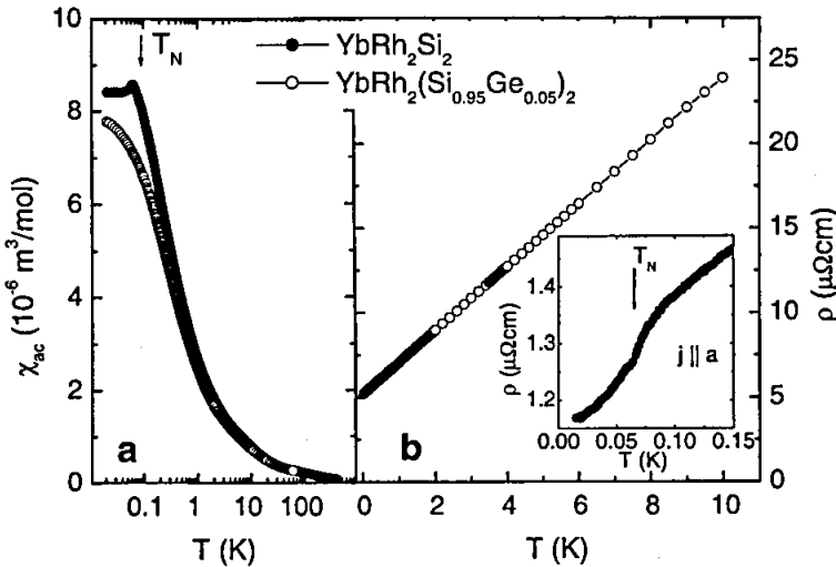
Fig. 4. (a) — ac magnetic susceptibility of \text{YbRh}_2(\text{Si}_{1-x}\text{Ge}_x)_2 ( x = 0 (●), x = 0.05 (○)) as \chi_{ac} vs T (on a logarithmic scale), measured along the tetragonal plane in zero dc-field. (b) — Electrical resistivity \rho of \text{YbRh}_2(\text{Si}_{0.95}\text{Ge}_{0.05})_2 showing a linear behavior \rho \sim T over a large temperature range 10 \text{ mK} \leq T < 10 \text{ K} . Inset: low-temperature electrical resistivity of pure \text{YbRh}_2\text{Si}_2 in zero field, arrow marks decrease at the Néel temperature.
