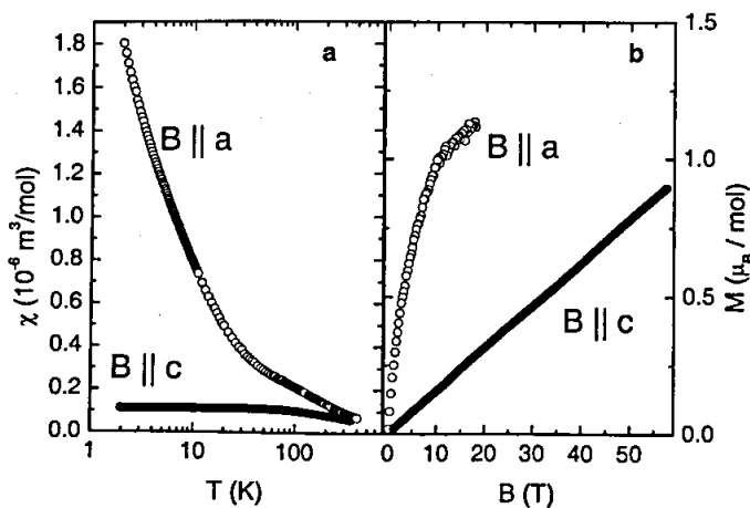
Fig. 1. Magnetic susceptibility \chi(T) = M/B vs T in B = 1 \text{ T} (a) and isothermal magnetization M vs B at 2 \text{ K} (b) for \text{YbRh}_2\text{Si}_2 in magnetic fields applied along the a - and c -axis ( \bullet ). Pulsed-field data in (b) for B \parallel c were taken on \text{YbRh}_2(\text{Si}_{0.95}\text{Ge}_{0.05})_2 and agree at least for B \leq 14 \text{ T} with those obtained from pure \text{YbRh}_2\text{Si}_2 .
