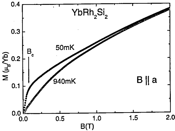
Fig. 2. DC magnetization M vs B for \mathbf{B} \parallel \mathbf{a} at two different temperatures T < T_N and T > T_N . The arrow marks the critical field B_c = 0.05 T.
