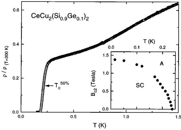
FIG. 8. Normalized resistivity \rho/\rho_{T=300\text{K}} for x=0.1 measured at zero field showing the SC transition at T_c^{50\%}=0.21 K. The inset shows the temperature dependence of the upper critical field B_{c2} separating the SC and A phases.
