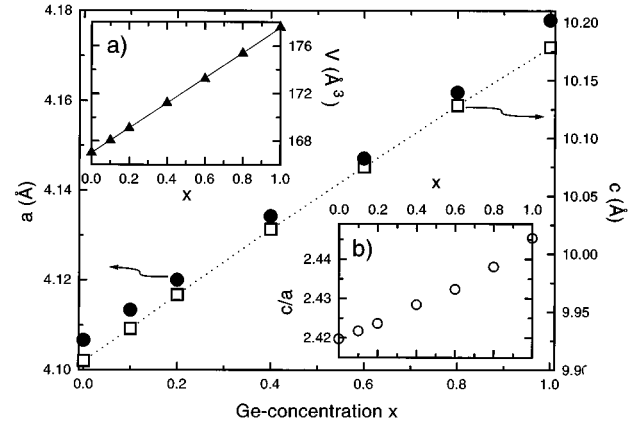
FIG. 1. Lattice parameters a (●) and c (□) of \text{CeCu}_2(\text{Si}_{1-x}\text{Ge}_x)_2 as a function of Ge concentration x . Insets: (a) unit-cell volume and (b) c/a ratio as a function of x . Lines are a guide to the eye.
