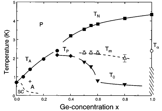
FIG. 9. ( T - x ) phase diagram of \text{CeCu}_2(\text{Si}_{1-x}\text{Ge}_x)_2 . Temperatures T_A , T_N , T_P , T_m , T_0 , and T_\alpha are described in the text. P , A , and SC indicate paramagnetic phase, A phase, and superconducting phase, respectively. Solid symbols indicate well-defined transitions of a different nature and open symbols are related to a change of regime. Lines are a guide to the eye. The hatched region accounts for irreversibilities present in \text{CeCu}_2\text{Ge}_2 (Ref. 25).
