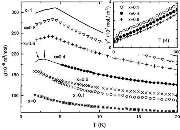
FIG. 3. Low-temperature magnetic susceptibility ( \chi ) measured in B=0.1 T for some \text{CeCu}_2(\text{Si}_{1-x}\text{Ge}_x)_2 concentrations. The arrows indicate both transitions observed in x=0.4 . Inset: high-temperature \chi^{-1}(T) for x=0.1, 0.4 , and 0.6 .
