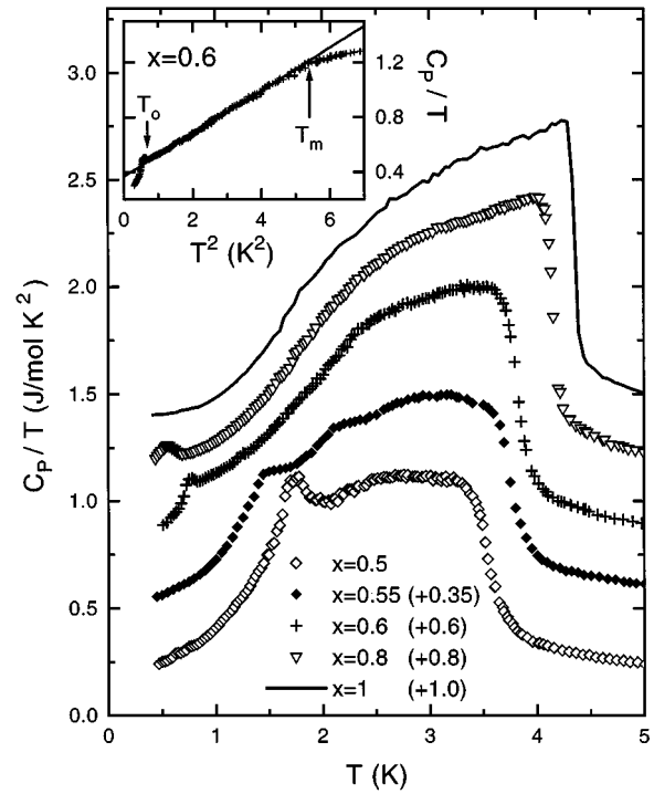
FIG. 6. Specific heat data of \text{CeCu}_2(\text{Si}_{1-x}\text{Ge}_x)_2 , in the high-concentration range as C_p/T vs T . For clarity the curves are shifted vertically by the amount indicated in parentheses. Inset: x=0.6 data in a C_p/T vs T^2 plot where the C_p \propto T^3 dependence, the kink at T_m , and the anomaly at T_0 are evident.
