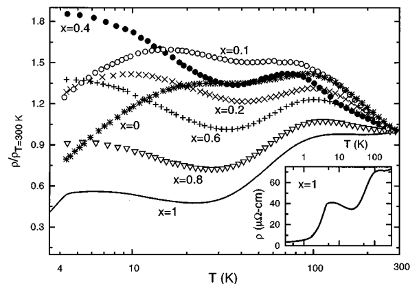
FIG. 2. Normalized resistivity \rho/\rho_{T=300\text{K}} of some \text{CeCu}_2(\text{Si}_{1-x}\text{Ge}_x)_2 studied samples as a function of temperature. Inset: \rho(T) for \text{CeCu}_2\text{Ge}_2 in a logarithmic scale.
