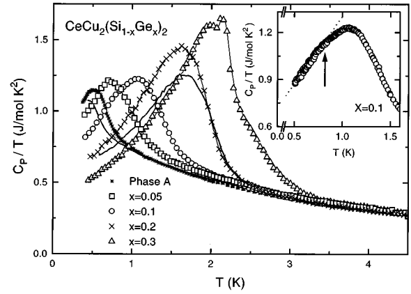
FIG. 4. Specific heat data of \text{CeCu}_2(\text{Si}_{1-x}\text{Ge}_x)_2 , in the low concentration range as C_p/T vs T . The data for x=0 and 0.2 in B=4 T are represented by a solid line. Inset: detail of x=0.1 at low temperature showing the kink at 0.8 K.
