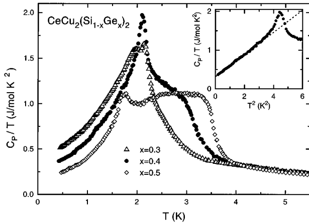
FIG. 5. Specific heat data of \text{CeCu}_2(\text{Si}_{1-x}\text{Ge}_x)_2 for intermediate concentrations in a C_p/T vs T plot. The inset shows the data for x=0.4 as C_p/T vs T^2 , which evidences the T^3 dependence.
