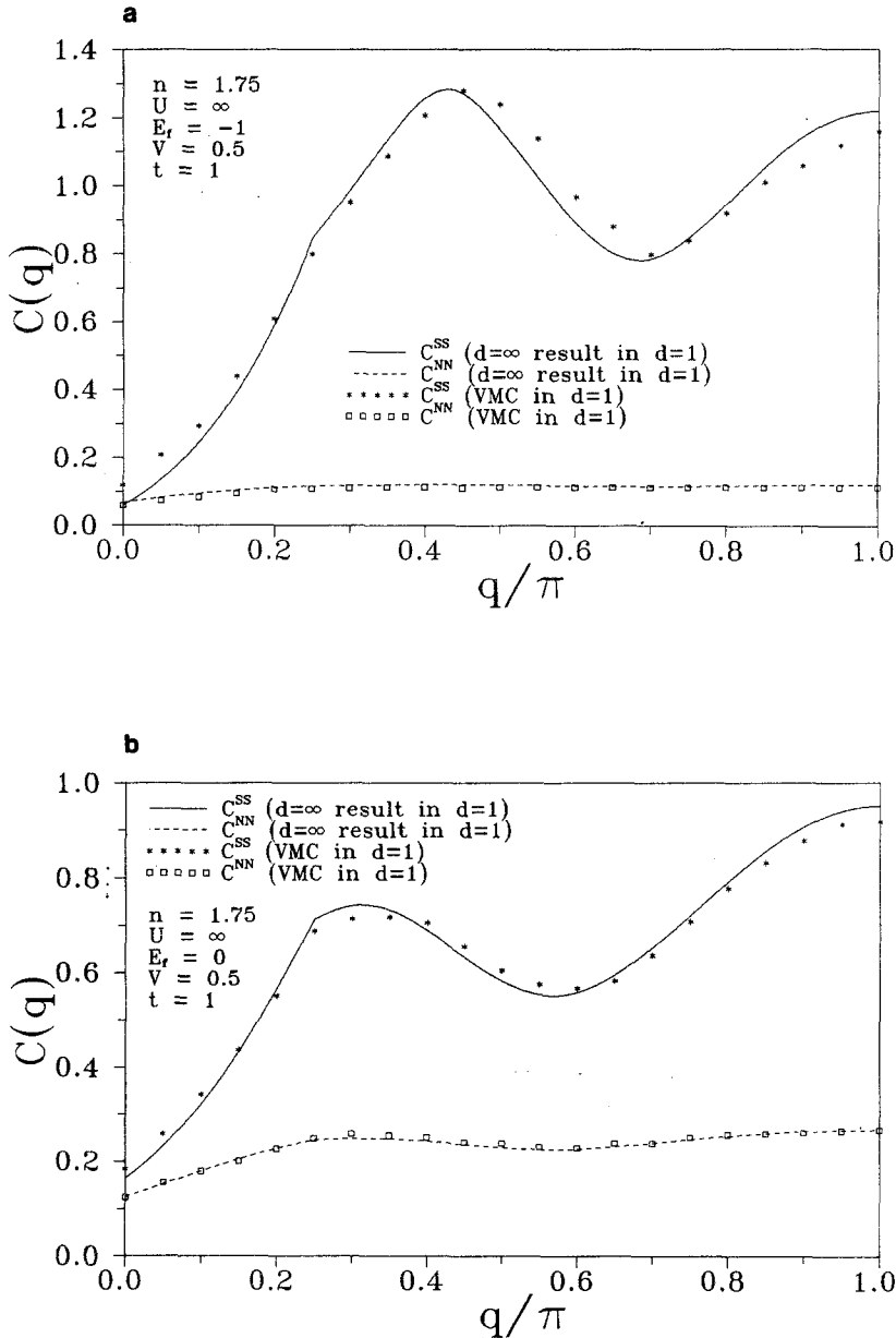
Fig. 6. Variational results for the momentum dependent spin-spin ( C^{SS} ) density-density ( C^{NN} ) correlation functions of the f -electrons in the d=1 periodic Anderson model for various parameter values of n and E_f . The numerical data of Shiba 18 are shown for comparison. (a) n=1.75 , E_f=-1 ; (b) n=1.75 , E_f=0 ; (c) n=2 , E_f=0 .
