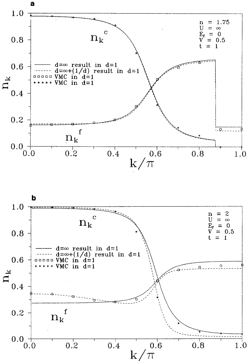
Fig. 5. Variational results for the momentum distributions n_k^c and n_k^f of the conduction and f -electrons, respectively, for the periodic Anderson model in d=1 . The numerical data by Shiba 18 are shown for comparison; (a) total density n=1.75 , (b) n=2.0 .
