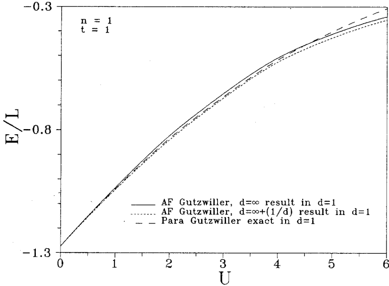
Fig. 3. Ground state energy of the Hubbard model versus U for different variational wave functions in d = 1 . The qualitative importance of the 1/d -correction for U \approx 4.5 is apparent (see text).
