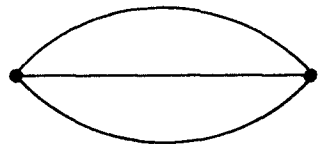
Fig. 1. Self energy diagram (second order) leading to 1/d -correction.
