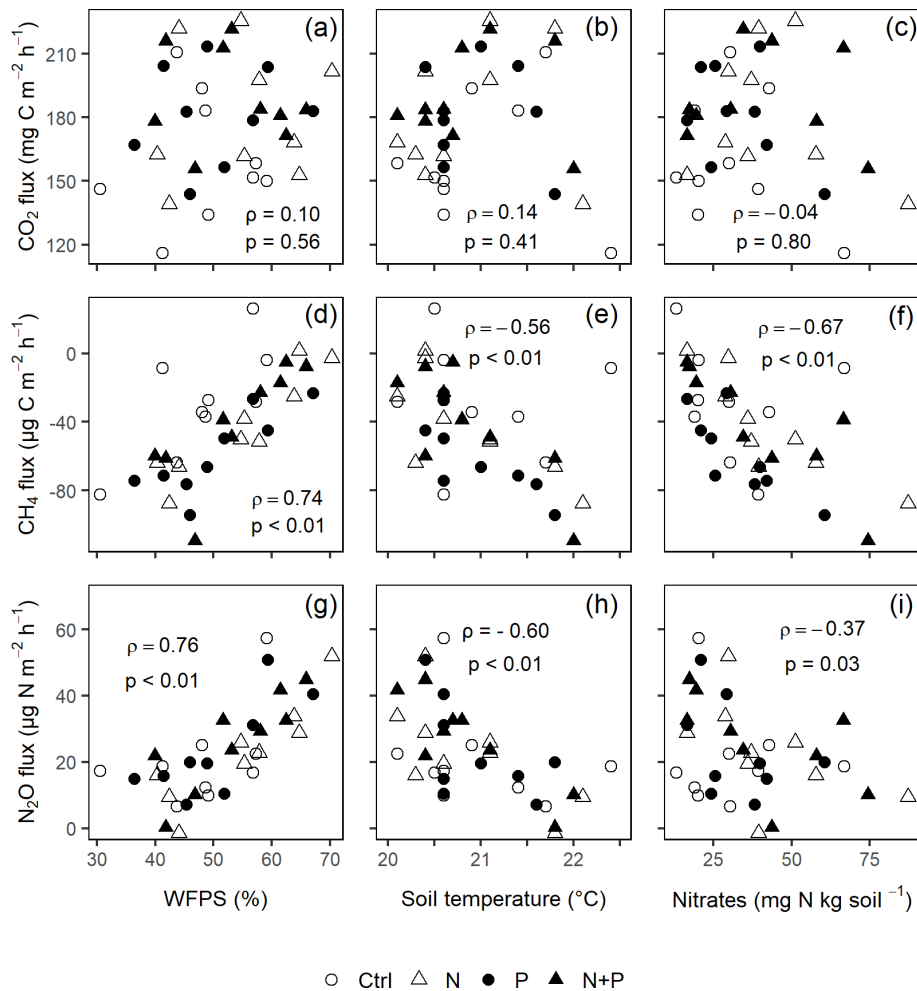
Figure 6. The Spearman correlation coefficient between mean background CO 2 (a–c), CH 4 (d–f), and N 2 O (g–i) fluxes and WFPS (column 1), soil temperature (column 2), and nitrates (column 3) using monthly measurement means of four replicate treatment plots (i.e., control (Ctrl), nitrogen (N), phosphorus (P), and N + P) taken between May 2019 and June 2020 ( p \leq 0.05 ; n = 16 ; i.e., four replicate plots in each of the four treatments). \rho is Spearman's correlation coefficient.
