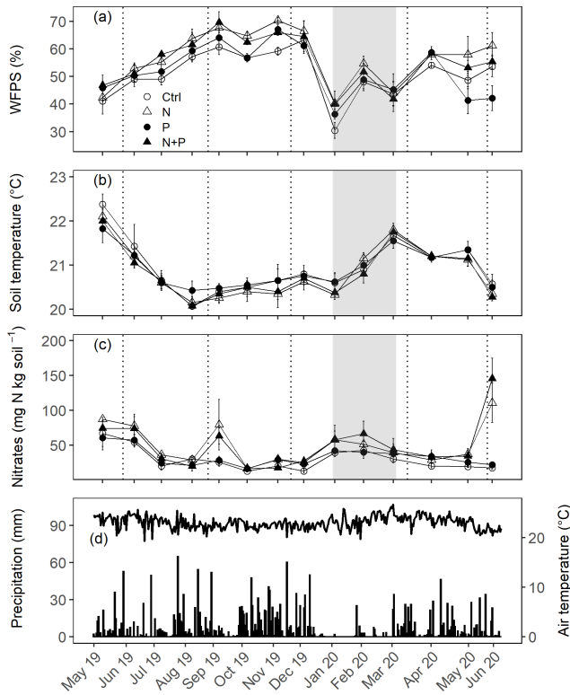
Figure 2. Mean ( \pm SE; n = 4 ) WFPS (a), soil temperature (b), and nitrates (c) in the top 0.05 m measured monthly (May 2019 to June 2020) from control (Ctrl), nitrogen (N), phosphorus (P), and N + P plots of the nutrient manipulation experiment. Vertical lines indicate the timing of each split dose of N ( 31.3 \text{ kg N ha}^{-1} ), P ( 12.5 \text{ kg P ha}^{-1} ), and N ( 31.3 \text{ kg N ha}^{-1} ) + P ( 12.5 \text{ kg P ha}^{-1} ) fertilization every 3 months. The gray shaded rectangle (in a, b, and c) marks the beginning and end of the dry season (January and February; monthly precipitation < 100 mm), while panel (d) gives the daily precipitation (bars) and air temperature (line) between May 2019 and June 2020. Climatic data were obtained from a weather station installed at the Budongo Conservation Field Station, 2 km from the location of the nutrient manipulation experiment in the Budongo Central Forest Reserve, northwestern Uganda.
