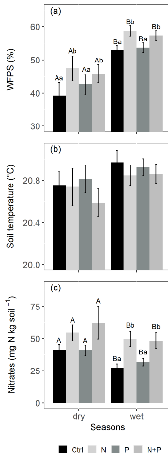
Figure 1. Mean ( \pm SE, n = 4 ) WFPS (a), soil temperature (b), and nitrates (c) in the top 0.05 m of the control (Ctrl), nitrogen (N), phosphorus (P), and N + P plots of the nutrient manipulation experiment measured during the dry (January and February; monthly precipitation < 100 mm) and wet (March to December; monthly precipitation > 100 mm) seasons. Different lowercase letters indicate the significant differences between treatments and the control, while different uppercase letters indicate significant differences between seasons (LMEMs; p \leq 0.05 ).
