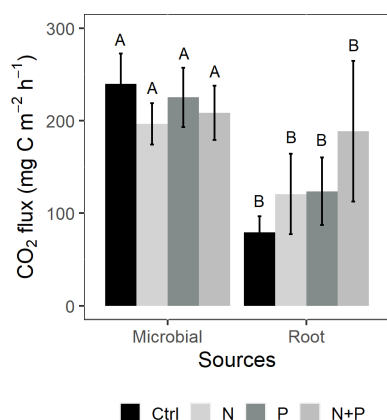
Figure 5. Mean ( \pm SE; n = 4 ) soil CO 2 flux from the control (Ctrl), nitrogen (N), phosphorus (P), and N + P plots of a trenching treatment separated into microbial and root sources. Different uppercase letters indicate significant differences between microbial and root contribution to total CO 2 flux (linear mixed effects models; p \leq 0.05 ).
