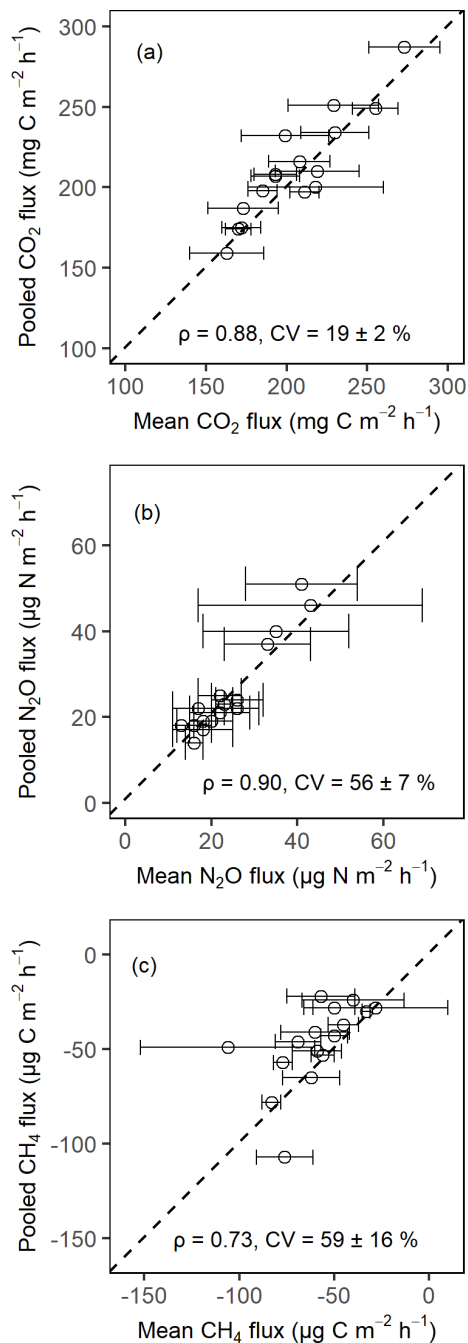
Figure A1. Comparison of the soil CO 2 fluxes (a), soil N 2 O fluxes (b), and soil CH 4 fluxes (c) from pooled sampling and the mean of four chamber measurements for the month of February 2020 in the Budongo Central Forest Reserve. \rho is the Spearman correlation coefficient, and CV is the coefficient of variation. Error bars are derived from standard error of the mean.
