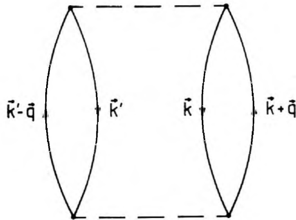
Fig.2: Second order Goldstone diagram.
