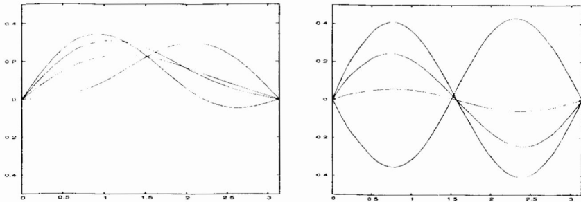
Figure 1 – Snapshot of the solution of the 4-mode truncation of (2.1) for \sigma = 2 (left) and for \sigma = 10 (right).
