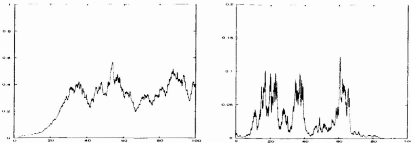
Figure 2 – First Fourier mode of the solution of the 4-mode truncation of (2.1) for \sigma = 2 (left) and for \sigma = 10 (right) for a single typical realization. It is clearly seen that 0 is stabilized (i.e., \sin destabilized) by large noise.
