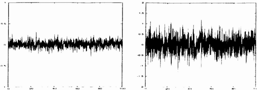
Figure 3 – Second Fourier mode of the solution of the 4-mode truncation of (2.1) for \sigma = 2 (left) and for \sigma = 10 (right) for a single typical realization. For \epsilon \rightarrow 0 one can show that it converges in a weak sense to white noise acting on \sin(2x) .
