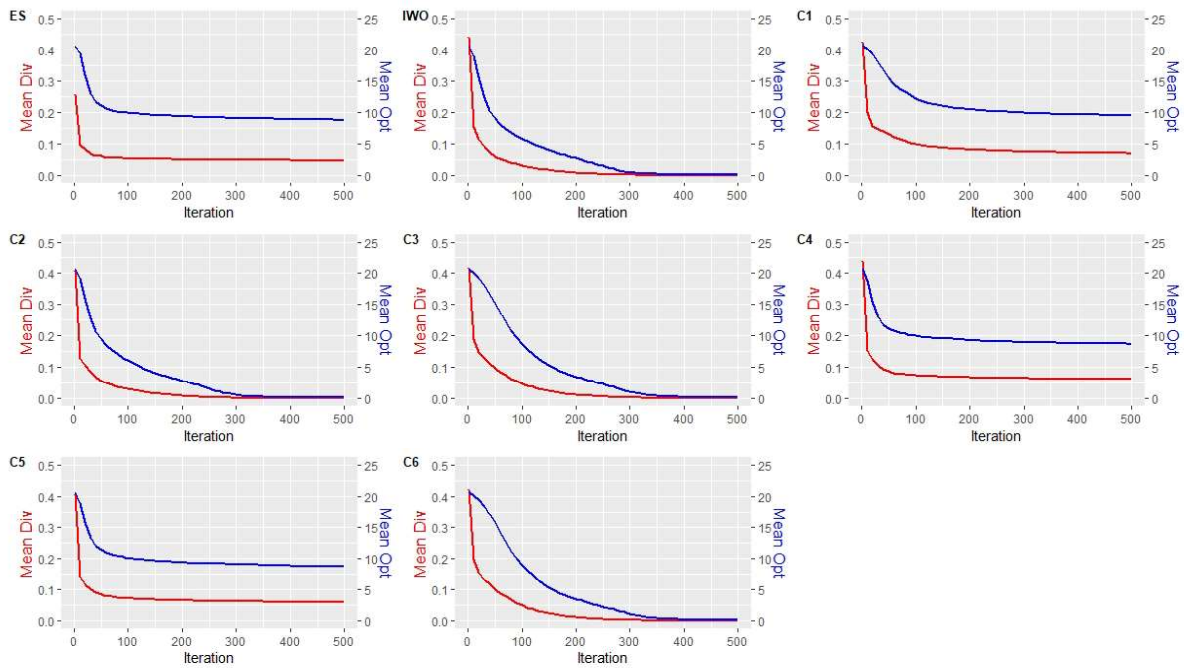
Figure 2: Progression of mean population diversity (Mean Div) and mean found optimum (Mean Opt) during the iterations of the runs for all combinations on the 30 dimensional Ackley function.
