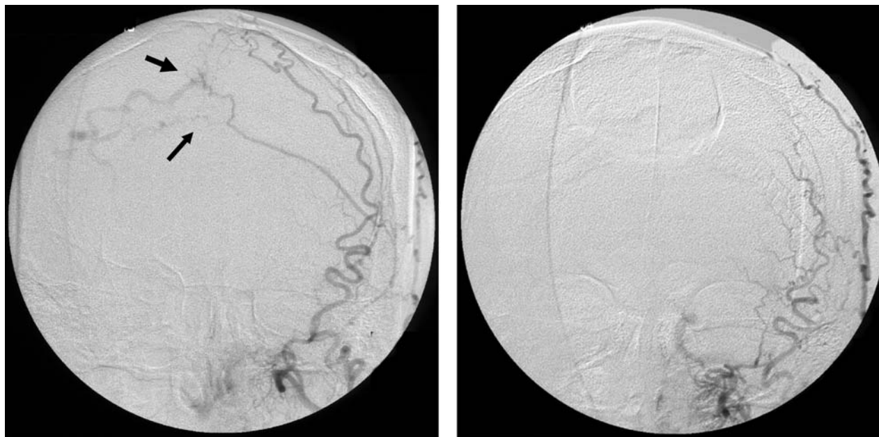
Fig. 2. Cerebral angiograms of a 60-year-old man with a right parietal parasagittal DAVF (Patient 6). (Left) Preoperative angiogram of left external carotid artery (anteroposterior view) showing drainage into the superior sagittal sinus and dilated elongated cortical veins. Note that there are two fistula points, one in the vicinity of the lambdoid suture and another very small fistula point 2–3 cm rostral to the suture (arrows). (Right) Postoperative angiogram with complete obstruction of the DAVF
