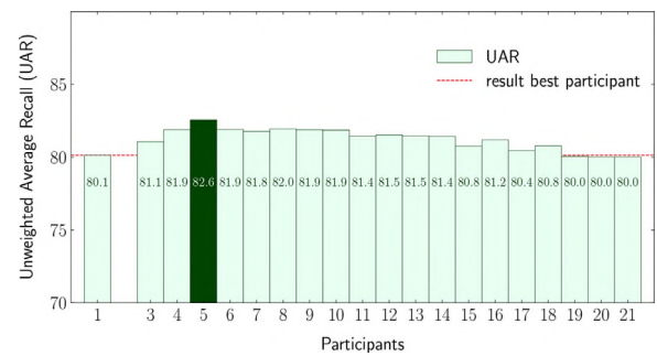
Fig. 5. Fusion results of the best n (1–21) approaches given by each participant following the final MSC ranking shown in Table 2. Fusion calculation only considers classification systems of the 21 participating teams (including not submitted/rejected papers) and not the original baseline system provided by Schuller et al. [38]. Position 2 is empty because in the case of a tie, the winning system is chosen. Best fusion (five systems) is given in dark green. (For interpretation of the references to colour in this figure legend, the reader is referred to the web version of this article.)
