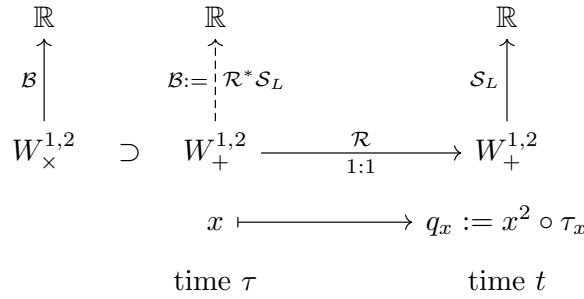
Fig. 1. Pull-back \mathcal{R}^* \mathcal{S}_L gives a formula \mathcal{B} that makes sense on a larger space on which critical points exist and represent time rescaled physical trajectories.
