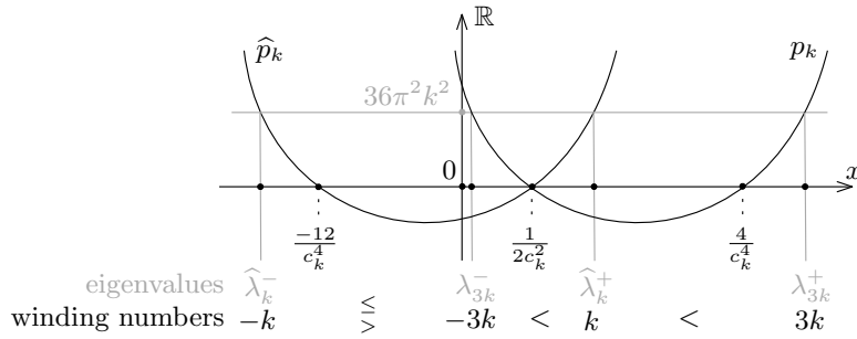
Fig. 5. The parabolas \widehat{p}_k and p_k , eigenvalues and winding numbers.
