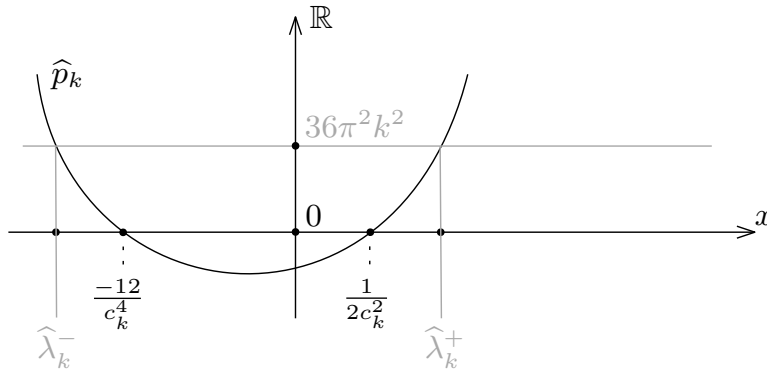
Fig. 4. Parabola \widehat{p}_k in the variable x = \widehat{\lambda}_k given by (45).
