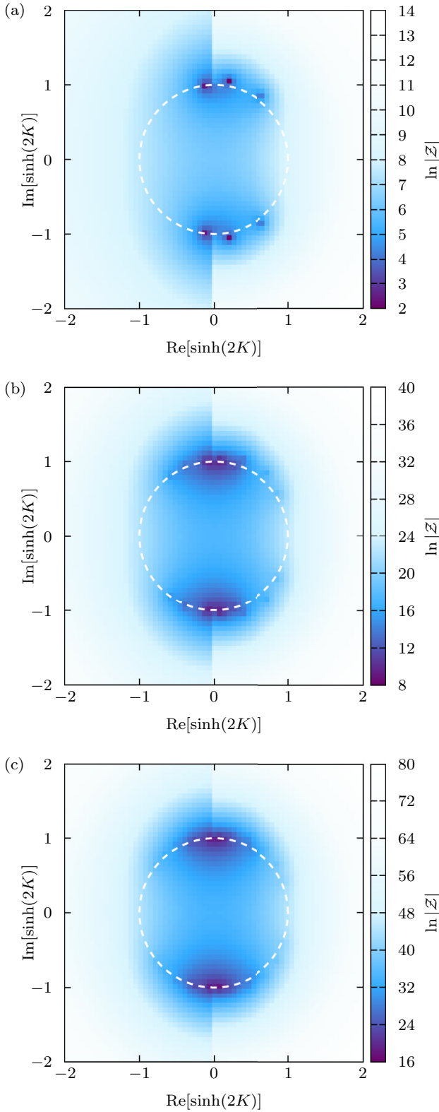
FIG. 3. Complex-partition-function zeros of Ising models on cylinders of different sizes: (a) 3 \times 3 , (b) 5 \times 5 , and (c) 7 \times 7 . With increasing system size, the distribution of Fisher zeros becomes denser. In the thermodynamic limit they will coalesce on the unit circle, indicated by the white dashed line.
