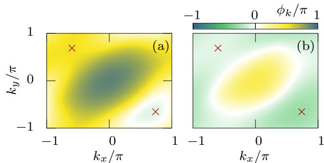
FIG. 3. Critical contours for the Haldane model with \phi = \pi/2 , V = 1 , and V' = 1/4 at nonzero initial temperature \beta = 1 . The red crosses mark the locations of the Dirac points of the two topological transitions at M_c = \pm 3\sqrt{3}V' . (a) Phase profile at time t = 1/2 for a topologically protected DQPT with a quench from m_i = 2 to m_f = 1/2 where the critical contour, along the white line here, encloses the Dirac point of the underlying crossed topological transition. (b) Phase profile at time t = 0.4 for a quench from m_i = 2 to m_f = -2 , starting and ending in the topologically trivial phase. Here, the critical contour separates two regions in the Brillouin zone either incorporating both Dirac points or none.
