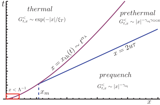
FIG. 1. Illustration of the spatiotemporal thermalization and prethermalization dynamics in terms of the fermionic Green's function G_{t,x}^< . For long distances x > 2ut and x > x_{\text{th}} , the Green's function is determined by the quasiparticles of the initial state and feature algebraic decay in real space corresponding to the prequench state of the system, modulated by an amplitude decaying as a stretched exponential in time. In the intermediate regime 2ut < x < x_{\text{th}}(t) , the corresponding quasiparticles correspond to the postquench Hamiltonian but are distributed according to a nonequilibrium distribution function, inducing a prethermal real-space scaling behavior |G_{t,x}^<| \sim |x|^{-\gamma_{\text{eq}}\gamma_{\text{GGE}}} . For short distances x < x_{\text{th}}(t) , the Green's function is thermal, \sim \exp(-|x|/\xi_T) , described by an effective temperature \tilde{T}_t and a corresponding thermal correlation length \xi_T . The scaling x_{\text{th}}(t) \sim t^{\alpha} , \alpha < 1 , implies that there exists a minimal distance x_m for which no clear prethermal regime can be identified since the scattering of quasiparticles is equally faster than the formation of quasiparticles. In this regime, the kinetic theory cannot be applied. The short-distance regime x < \Lambda^{-1} , for which Luttinger theory is invalid, occupies a negligibly small short-time regime.
