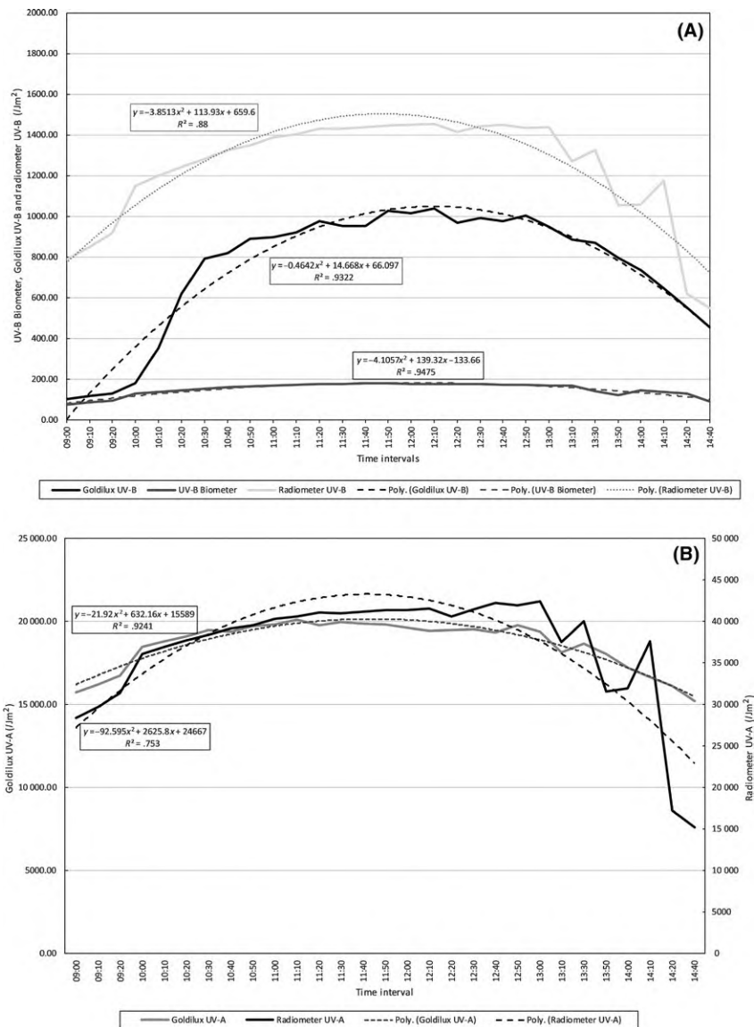
FIGURE 3 Diurnal pattern in UV-B (A) and UV-A (B) measurements from the biometer, radiometer and Goldilux on the 19th January 2017. Missing data and cloud-affected values have been removed at 09:30, 09:40, 09:50, 13:20, 13:40 and 14:30. The maximum UV-B biometer reading was ~180.00 J m -2 and the maximum Goldilux UV-B reading was 1000.00 J m -2 . The maximum radiometer UV-A reading was ~42 000.00 J m -2 and the maximum Goldilux UV-A reading was ~20 000.00 J m -2
