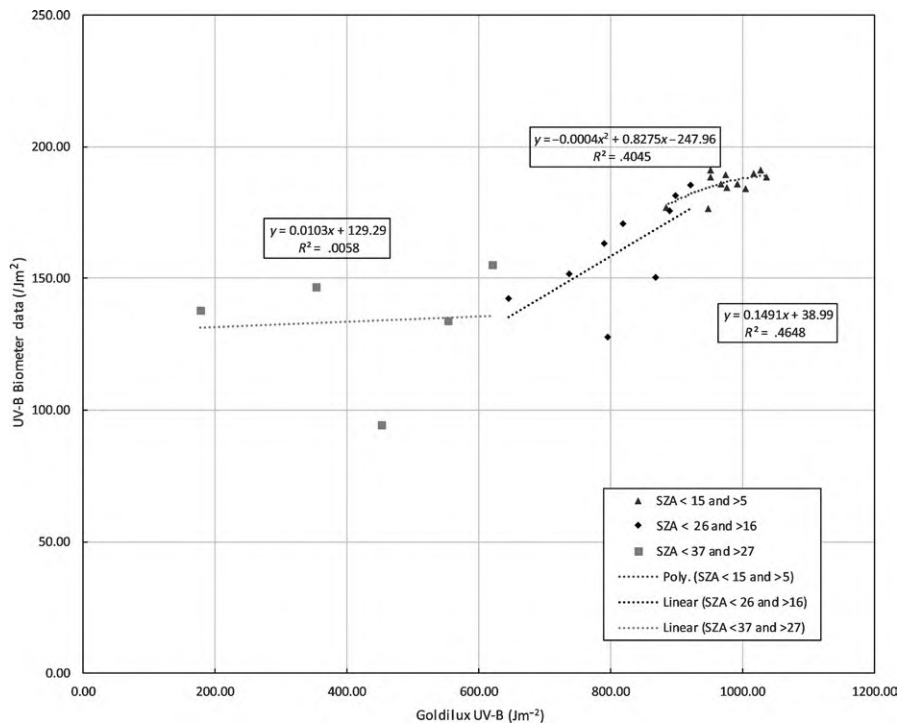
FIGURE 4 Correlation between UV-B biometer UV-B data and Goldilux UV-B data by SZA category: 5°-15° (sun high in the sky), 16°-26° and 27°-37° (sun closest to the horizon)
