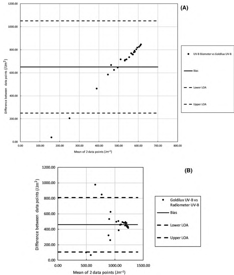
FIGURE 6 Bland-Altman plot for UVB from the (A) UV-B biometer and Goldilux and (B) radiometer and Goldilux comparing the difference between measurements graphically plotted against the means
