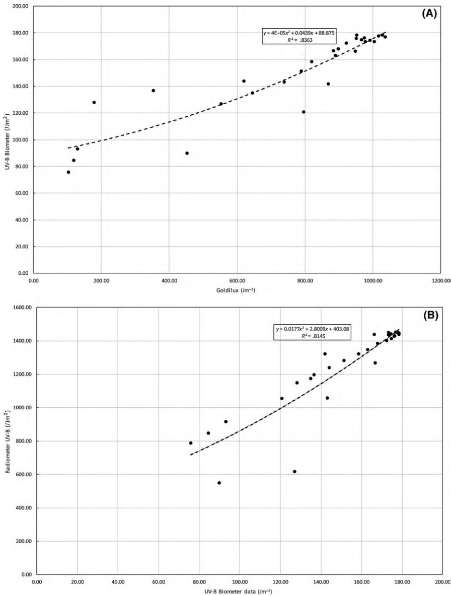
FIGURE 5 Correlation between UV-B measurements from (A) Goldilux and from the UV-B biometer, and (B) biometer and the radiometer at all of the time intervals with data available
