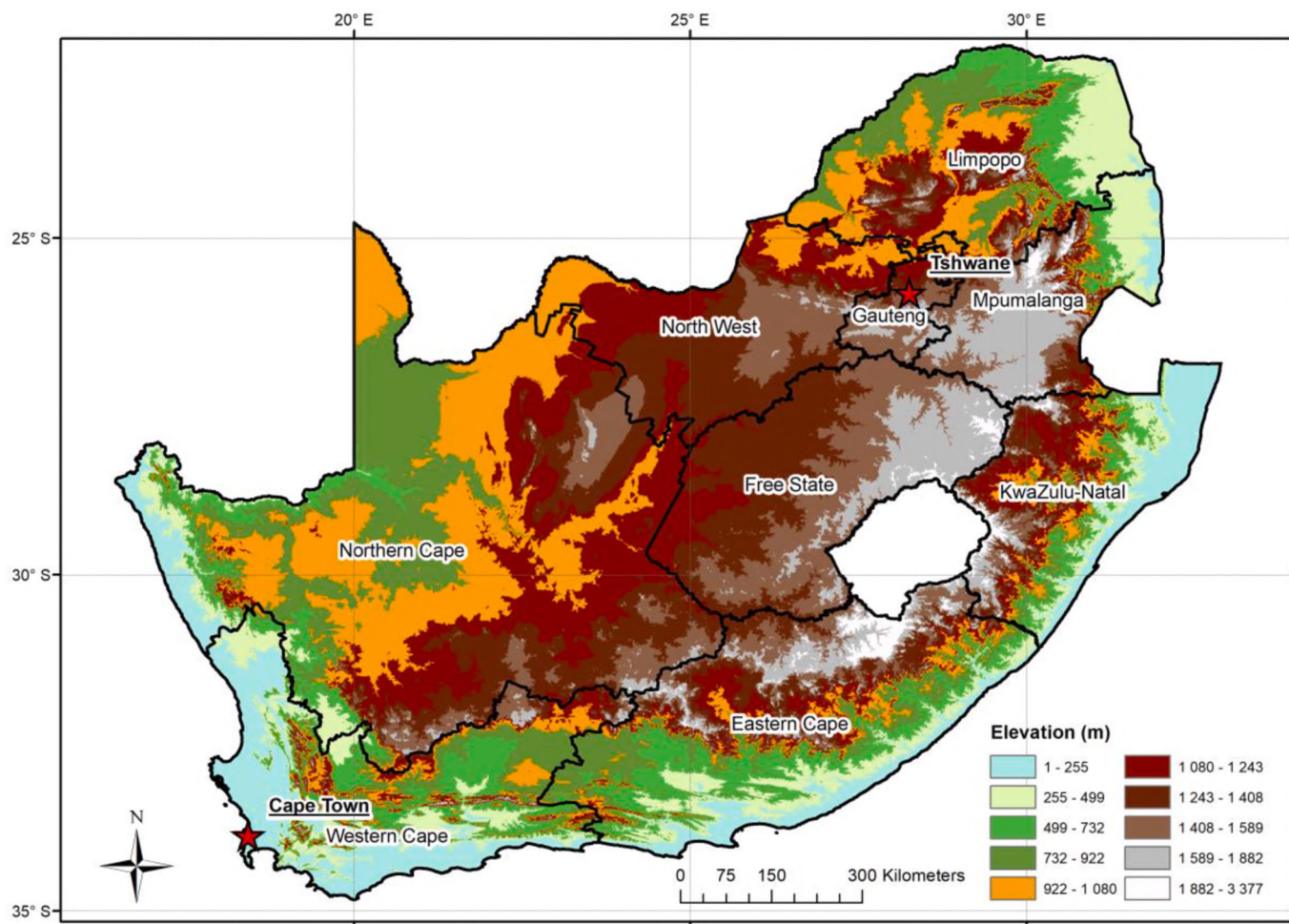
Fig. 1. The topography and provinces of South Africa.
