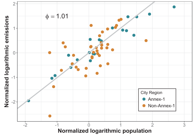
Fig. 1. Scaling of CO 2 emissions with population size for 61 global cities. The data has been normalised by subtracting average logarithmic values, see Section 3. The solid grey line is the regression obtained from the Reduced Major Axis (RMA, Section 2) and the slope is \phi \approx 1.01 , see Table 1 for details.
