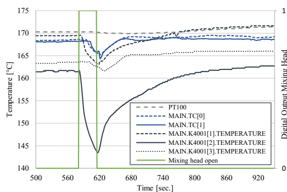
Fig. 3 (a): Flow front detection with temperature sensors
