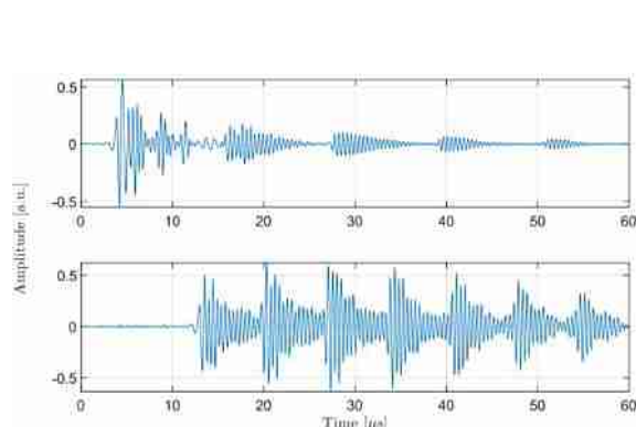
Fig. 4 (a): Ultrasonic signals. At the top, the pulse-echo signal, at the bottom the corresponding transmission signal.
