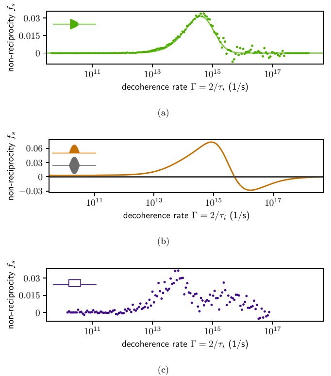
FIG. 4. Nonreciprocity of the devices introduced in Fig. 3 calculated with the Lindblad formalism (continuous lines) and the Monte Carlo wave function method (dotted). (a) Nonreciprocal transport through the device A [Fig. 3(a)] occurs for 5 \times 10^{12} < \Gamma < 3 \times 10^{15} \text{ s}^{-1} . As anticipated, both methods yield coincident results. The Monte Carlo data was obtained from 6.4 \times 10^6 realizations of the time evolution. (b) Nonreciprocal transport of device B [orange, Fig. 3(b)] in the transition regime and return to reciprocal behavior for large and small \Gamma . The transport through the symmetric device D [gray, Fig. 3(d)] is fully reciprocal, however. (c) Nonreciprocal transmission of device C [Fig. 3(c)] as obtained with the Monte Carlo wave function method.
