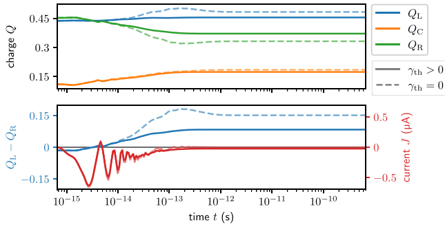
FIG. 16. Plots showing the time evolution of charges and currents in the open nine-site chain with additional jump operators that are specifically chosen to drive the system towards the state given by the thermal density matrix (see Appendix C3). The rate \gamma of the wave-packet generating jump operators and the rate \gamma_{\text{th}} of the additional thermalizing jump operators are given by \gamma = 1.5 \times 10^{15} Hz and \gamma_{\text{th}} = 3 \times 10^{14} Hz, respectively. The steady-state charge imbalance indicates that the novel steady state persists even in the presence of thermalizing processes. The dashed lines show the case without the additional jump operators, which is the same data as shown in Fig. 7(a).
