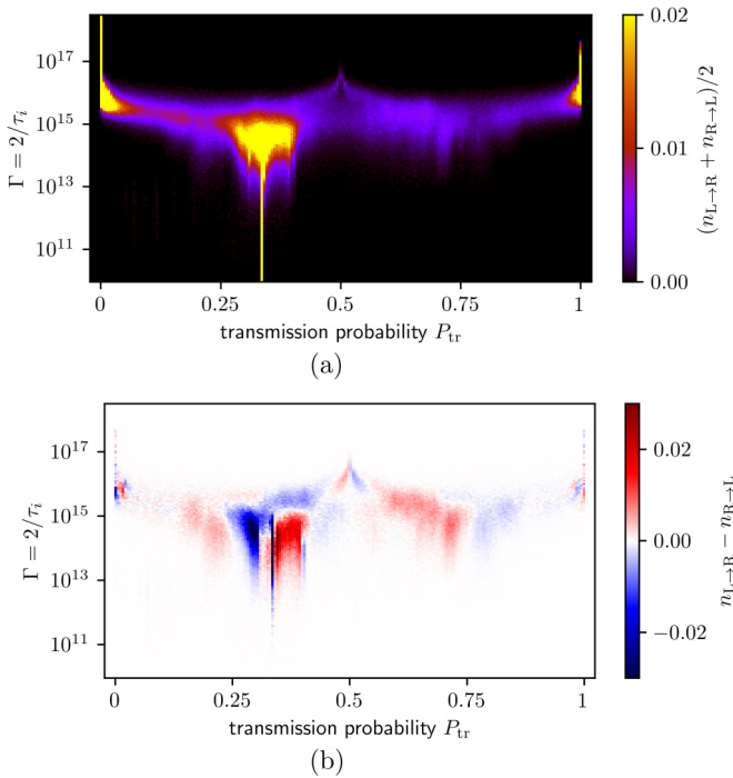
FIG. 5. Color maps showing the transmission probability distribution as a function of P_{tr} and decoherence rate \Gamma for device A. (a) The direction-independent mean of the distributions for L \rightarrow R and R \rightarrow L directions illustrate the different transport regimes. (b) The difference of the distributions for the two directions shows the direction dependent effect of decoherence, which leads to nonreciprocal dynamics on long time scales in the transition regime.
