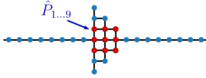
FIG. 11. Sketch of the tight-binding implementation of device A. The circles represent the system sites and the red sites correspond to inelastic scattering centers. These centers mediate the coupling to the environment.
