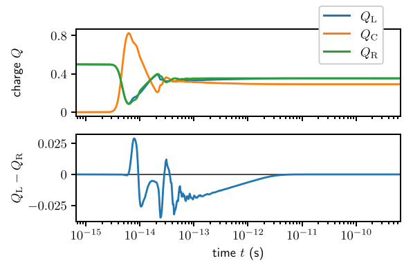
FIG. 15. Plots showing the time evolution of charges in the device with longitudinal asymmetry [Fig. 3(a)] as calculated using Eq. (3). The upper panel shows the total charge Q_L in the left lead, in the right lead Q_R , and within the central device Q_C . The bottom panel shows the charge difference between the left and right leads, which is zero for large and small times. For intermediate times, however, the difference is finite, revealing a transient charge separation.
