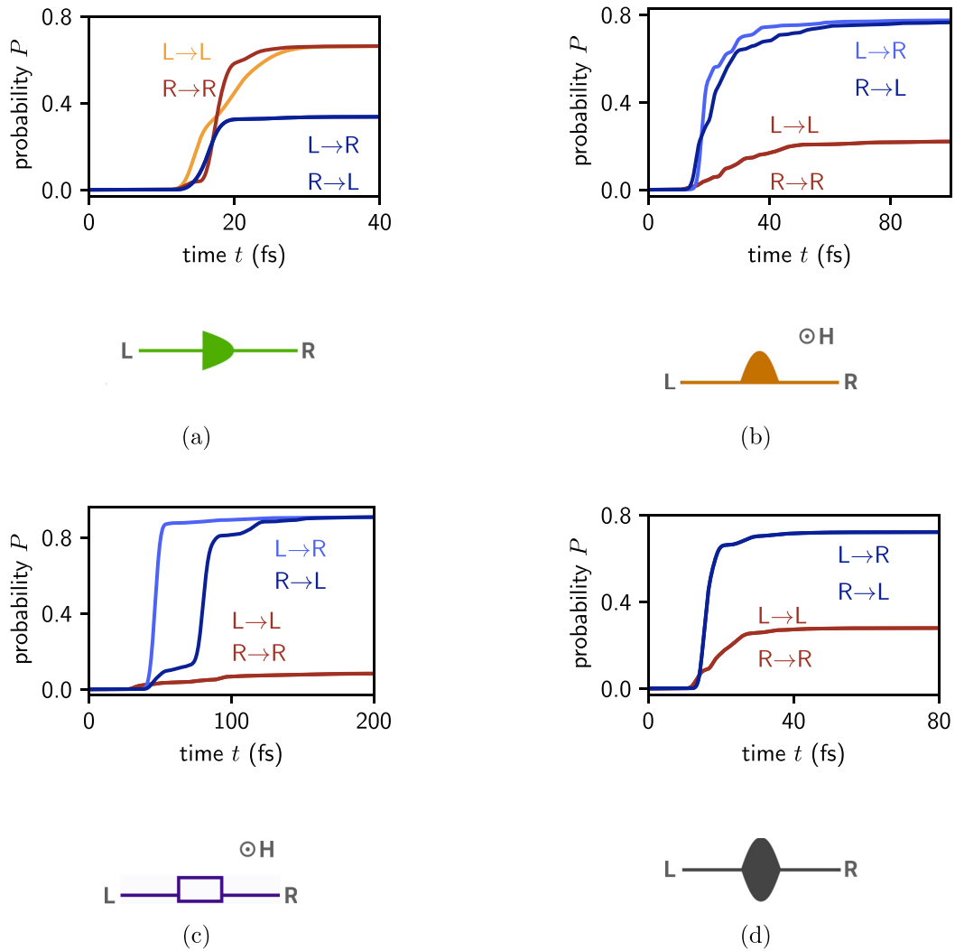
FIG. 3. Layouts and time resolved transmission and reflection probabilities of unitary conductors with (a) a longitudinal asymmetry, (b) a transversal asymmetry, (c) an asymmetric Aharonov-Bohm loop, and (d) a symmetric device. The devices (b) and (c) with areas 28 a^2 and 398 a^2 are penetrated by magnetic fluxes \Phi = 1.4 and 0.4 h/e , respectively, where a = 0.3 nm is the unit length of the tight-binding lattice and h/e is the magnetic flux quantum. The structures connect two ports L and R . In the plots, the transmission probabilities P_{m \rightarrow n} for electrons emitted as Gaussian wave packets ( k_0 = \pi/3a , \sigma_x = 0.9 nm for (a), (b), (d) and 24 nm for (c)) by port m to reach port n calculated as a function of time after emission are presented for the scattering-free, unitary transport. The devices' lengths are (a) 1.8 nm, (b) 3.0 nm, (c) 12 nm, and (d) 2.4 nm.
