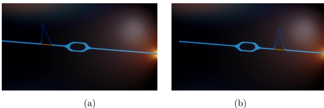
FIG. 9. (a) Unitary propagation of a wave packet (blue) across an asymmetric Aharonov-Bohm ring (gold) biased with a magnetic flux penetrating the hole of the ring. The wave packet, presented as |\psi(r, t)|^2 , arrives from the left and passes the ring in a straightforward manner. The data have been obtained by exact diagonalization as described in the main text. (b) The wave packet arriving from the right passes the ring only after having been reflected back and forth.
