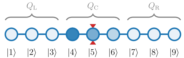
FIG. 6. Sketch of the tight-binding chain used for most of the calculations in Sec. IV. The blue circles represent the tight-binding sites. The fill color of the sites sketches the local value of the electrostatic potential. The darker the shade, the higher is the potential at that site. The sites |4\rangle , |5\rangle , and |6\rangle implement an asymmetric potential barrier. The central site |5\rangle highlighted by the red arrows is coupled to a trap, which may absorb the particle and release it again as a wave packet. The observables Q_L , Q_R , and Q_C are used to measure the charge density in the left, right, and central region of the open system shown, respectively.
