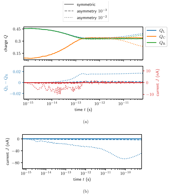
FIG. 14. Plots of the time evolution of charges in the open system as shown in Fig. 6, but with fully symmetric (solid lines) and slightly asymmetric (dashed and dotted lines) potential barriers. The dashed line corresponds to a barrier similar to Eq. (C7) but with the potentials 1.999t, 2t, 2.001t at sites |4\rangle, |5\rangle, |6\rangle . The dotted line corresponds to potentials 1.99t, 2t, 2.01t at sites |4\rangle, |5\rangle, |6\rangle . (a) While no charge separation occurs in the fully symmetric open system, charge separation starts to occur with increasing barrier asymmetry. (b) No persistent current is flowing in the fully symmetric shorted system. Again, with increasing barrier asymmetry, persistent currents occur. The calculational method used is completely identical with the one used in Fig. 7, the only difference being the symmetry of the barrier. Some of the blue Q_L curves are not visible because they fully overlap with the corresponding green Q_R curves.
