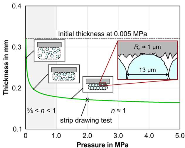
Fig. 7 Thickness-pressure curve of one fiber layer for the compression of three layers twill woven fabric 280 \text{ g/m}^2 and schematic overview of the compression behavior of one fiber roving in contact with the metal sheet
