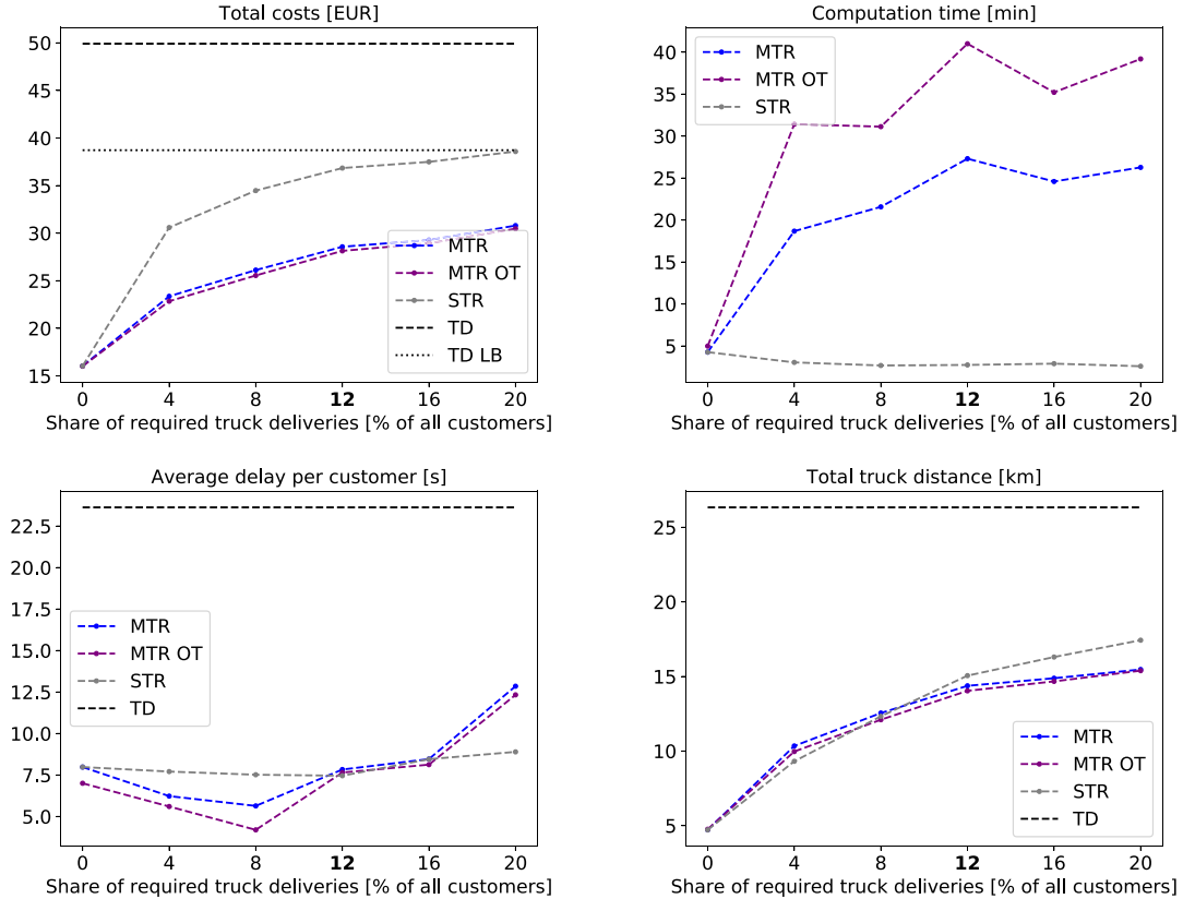
Fig. 8. Comparison of different delivery modes for a varying share of required truck deliveries.
