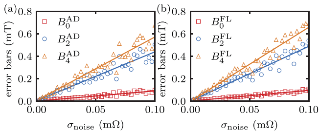
FIG. 6. Error bars of the extracted SOT parameters in the presence of experimental noise \sigma_{\text{noise}} . The simulation input parameters are listed in Table II, and \sigma_{\text{noise}} was added to the simulated first and second harmonic signals (see Fig. 2, sampled in 1 mT steps). Panels (a) and (b) show the results and linear fits for B_{0,2,4}^{\text{AD}} and B_{0,2,4}^{\text{FL}} , respectively.
