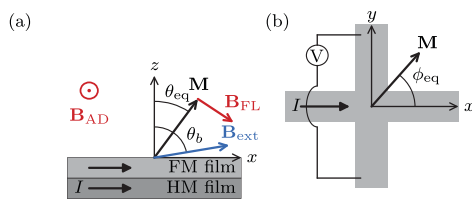
FIG. 1. Geometry and coordinate system. (a) Side view of the Hall bar structure. \mathbf{M} is the magnetization, and \mathbf{B}_{\text{ext}} the external applied field. \theta_{\text{eq}} and \theta_b are the azimuthal angles of the magnetization and external applied field from the z-axis, respectively. \mathbf{B}_{\text{AD}} , \mathbf{B}_{\text{FL}} are the effective SOT fields. (b) Top view of the Hall bar structure indicating the in-plane angle \phi_{\text{eq}} of the magnetization, as well as the measurement direction of the transverse voltage.
