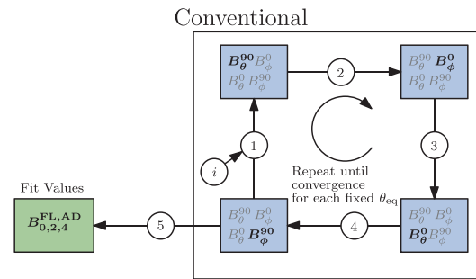
FIG. 3. Flow chart of the conventional iterative procedure to extract spin-orbit torques from harmonic measurements. The steps, indicated by the encircled numbers, are explained in the text. The updated quantities are printed in bold. Note that the fit of the desired torque coefficients is performed only once, after the boxed loop has reached convergence.
