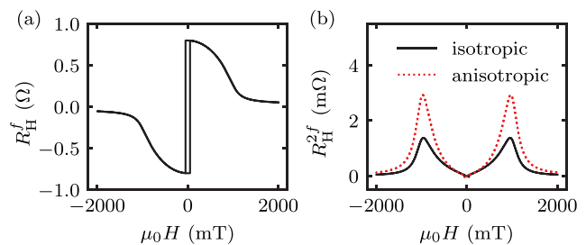
FIG. 2. Expected (a) first harmonic signal R_{\text{H}}^f and (b) second harmonic signal R_{\text{H}}^{2f} , the latter with and without higher order coefficients at \phi_{\text{eq}} = 90^\circ and \theta_b = 88^\circ . For the simulated SOT parameters, see Tables I and II.
