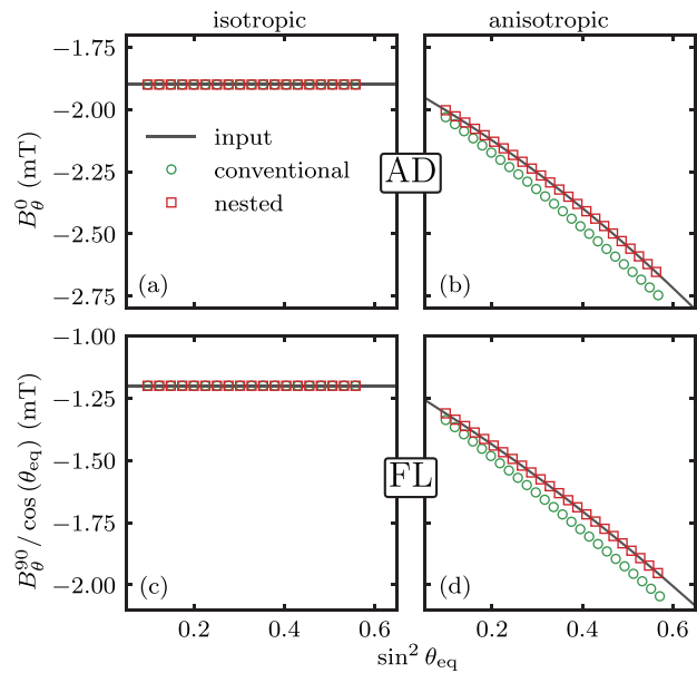
FIG. 5. SOT fields extracted from the conventional and nested iterative analysis as a function of magnetization angle \sin^2 \theta_{eq} . (a) and (c) show the results for the isotropic SOTs (see parameters in Table I). (b) and (d) show the fields extracted from the anisotropic SOT simulation (see Table II). The functional dependence expected from the known input parameters is plotted with solid lines. The extracted torque coefficients are listed in Tables I and II.
