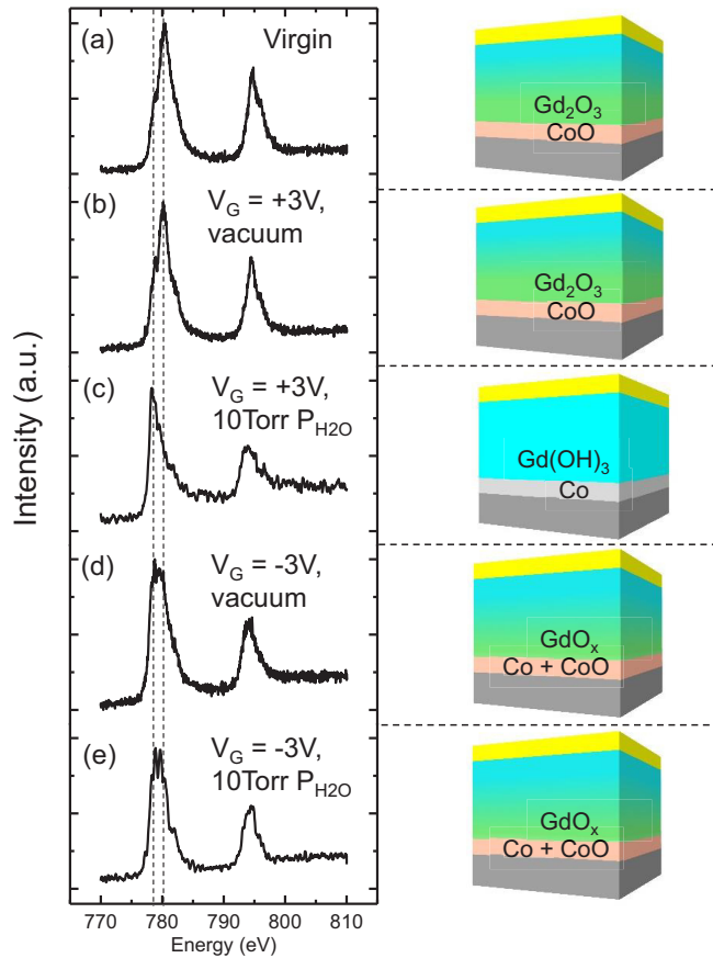
FIG. 5. (a)–(c) XAS spectra of Mg(30nm)/Pd(10 nm)/Co(0.9 nm)/GdO x (30 nm)/Au(3 nm) device in virgin state (a) and after V_G = +3 V was applied for 600 s in vacuum (b) and in 10 Torr of P H 2 O (c), respectively. The experiments from (a) to (c) were done sequentially. (d), (e) XAS spectra of the device in (c) after V_G = -3 V was applied for 600 s in vacuum and in 10 Torr of P H 2 O , respectively. Two different devices in (c) were used for experiments in (d) and (e).
