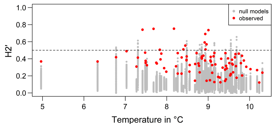
FIGURE 2 Scatterplot of observed H_2' (red dots) and randomized H_2' values (gray dots) along a mean multi-annual temperature gradient. Dashed horizontal line indicates H_2' = 0.5 . A null model calculated randomized H_2' values with 1000 simulations (in 87% of the networks, the observed H_2' was significantly higher than in random assemblages).
