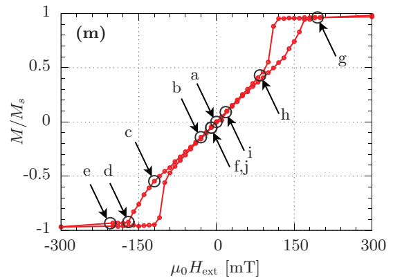
FIG. 2. (Color online) (a)–(l) Selection of magnetization images of a 750 nm diameter CoB/Pt disk at various out-of-plane magnetic field steps, where white indicates magnetization pointing up (positive field direction) and black indicates magnetization pointing down. (a) shows the virgin state after deposition. Between (a) and (b), the sample experienced a field of 65 mT. Between (e) and (f), between (g) and (h), and between (i) and (j), the sample was saturated. (k) visualizes the difference of (d) and (e), and (l) depicts the sum of (d) and (g), highlighting the different positions of the bubbles in these images. (m) shows an out-of-plane hysteresis loop of a continuous CoB/Pt film, in which the field values corresponding to images (a)–(l) are illustrated.
